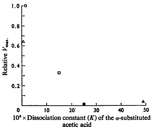
Fig. 7. Correlation between the relative V_{\max} for some C-2-substituted D-glucose 6-phosphates and the dissociation constants of the correspondingly substituted \alpha -substituted acetic acids
