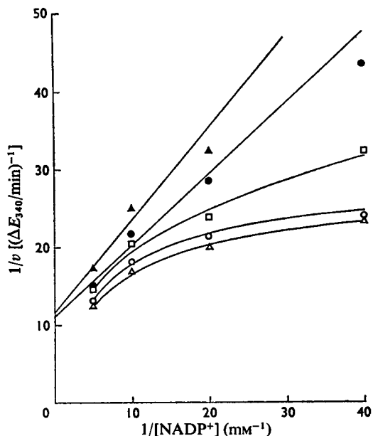
Fig. 5. Yeast glucose 6-phosphate dehydrogenase: variation of the reciprocal of the initial rate with the reciprocal of the NADP^+ concentration for several concentrations of 2-deoxy-D-arabino-hexose 6-phosphate
