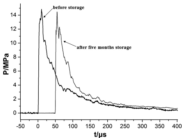
Figure 2. Pressure-time curves of the GM-MgH 2 sensitized emulsion explosive, before and after storage.
