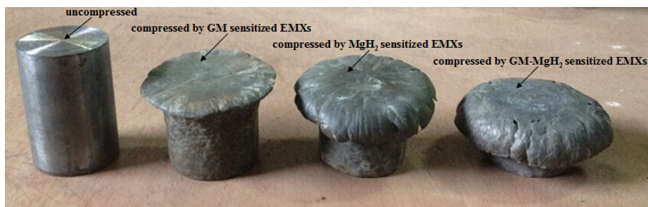
Figure 3. Power of different emulsion explosives characterized by the compression of a lead block.
