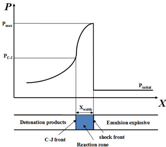
Figure 4. Schematic diagram of the ZND detonation model.
