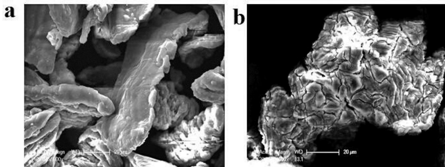
Figure 1. Micrograms of MgH 2 powders: (a) untreated; (b) coated with paraffin.
