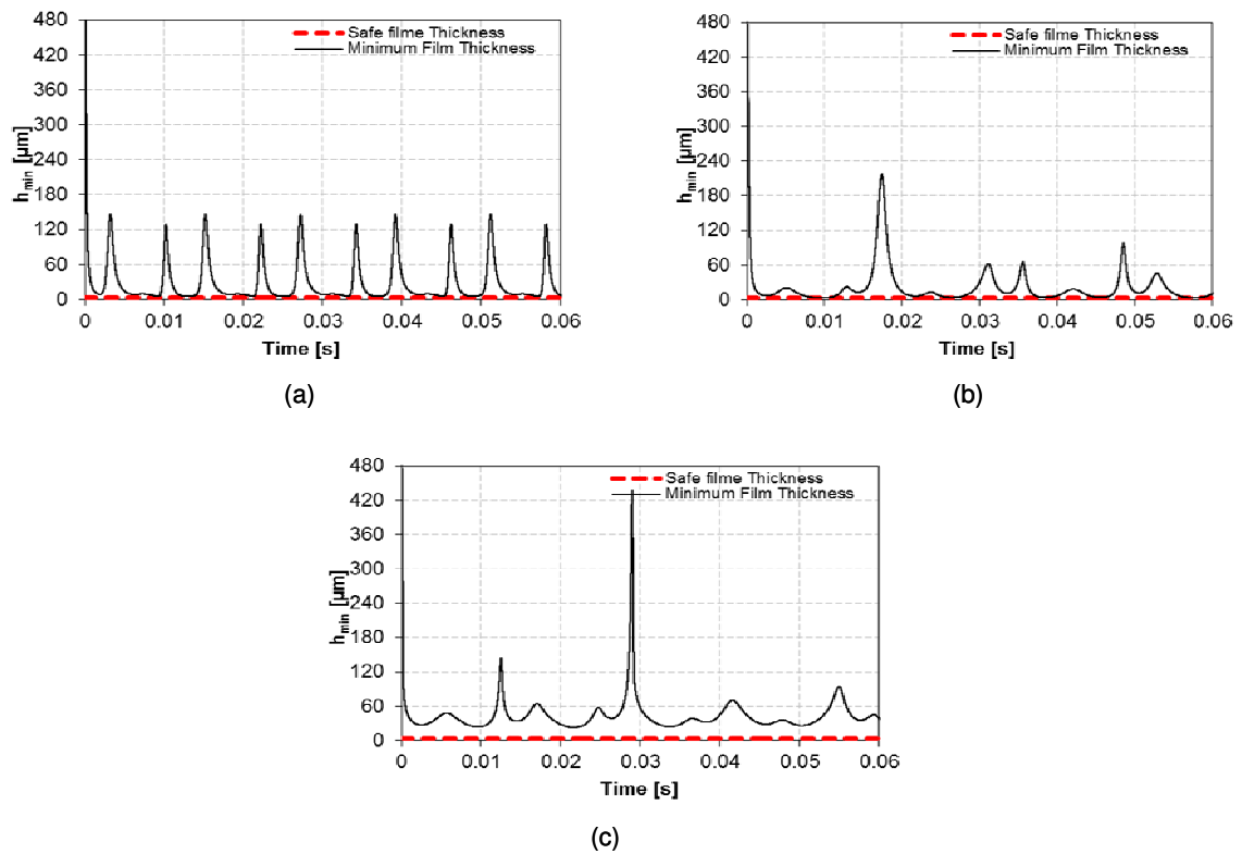
Fig. 20 Minimum film thickness for different lubrication models: (a) Pinkus and Sternlicht; (b) Frêne et al. (long); (c) Frêne et al. (short)
