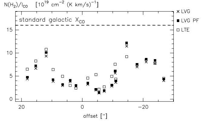
Fig. 10. Variation of X_{\text{CO}} across the analyzed positions in M82. Offsets are given relative to the center of M82 ( 2.2 \mu\text{m} peak). The \text{H}_2 column densities were derived using the LTE, the LVG and \text{LVG}_{\text{PF}} solutions. The dotted line at X_{\text{CO}} = 1.6 \cdot 10^{20} \text{ cm}^{-2} (\text{K km s}^{-1})^{-1} corresponds to the standard Galactic conversion factor
