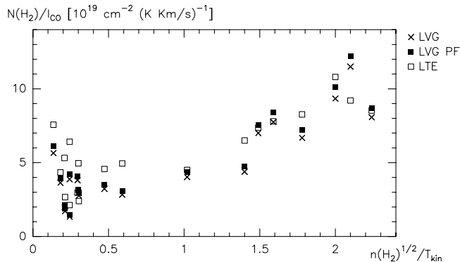
Fig. 11. X_{\text{CO}} as derived from the LTE, LVG and LVG PF solutions versus T_{\text{kin}}^{-1} n(\text{H}_2)^{1/2} . The plot shows a linear correlation between the conversion factor and the associated \text{H}_2 densities and kinetic temperatures beyond T_{\text{kin}}^{-1} n(\text{H}_2)^{1/2} \approx 0.5
