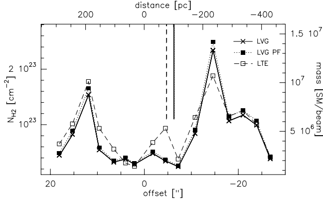
Fig. 9. Beam averaged \text{H}_2 column densities across the major axis of M82. Offsets are given relative to the center of M82 ( 2.2 \mu\text{m} peak). The thick solid line corresponds to the \text{H}_2 column densities derived from the LVG solutions. The dashed and the dotted lines give the corresponding values for the LTE approximation and the solution calculated from the partition functions ( \text{LVG}_{\text{PF}} ), respectively. The vertical lines indicate the location of the centroid of mass of the three \text{H}_2 distributions. Note that the location of the centroid of mass is identical for the LVG and \text{LVG}_{\text{PF}} solution. The labeling of the right axes gives the \text{H}_2 mass per beam in units of solar masses
