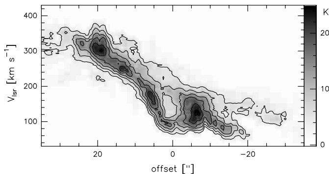
Fig. 3. A pv -diagram along the major axis of M82 in the ^{12}\text{CO}(J = 2 \rightarrow 1) transition. The contours correspond to 4, 8, 12, 14, 18, and 22 K. The pv -diagram is centered on the brightest radio continuum point source SNR 41.9+58 (see Figs. 1 and 2). The velocity crowded regimes at 20'' , 5'' and -7'' offset correspond to the western, central and eastern CO peak
