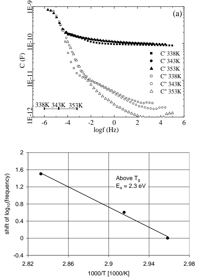
Figure 9: (a) Master plot based on low-frequency dielectric behavior for dry n3 ; (b) Arrhenius plot indicating charge transport activation energy
