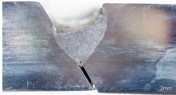
Fig. 3. Tekken sample W2. Welding bead performed underwater with heat input 1.1 kJ/mm. No imperfections. Beracha's etch.
