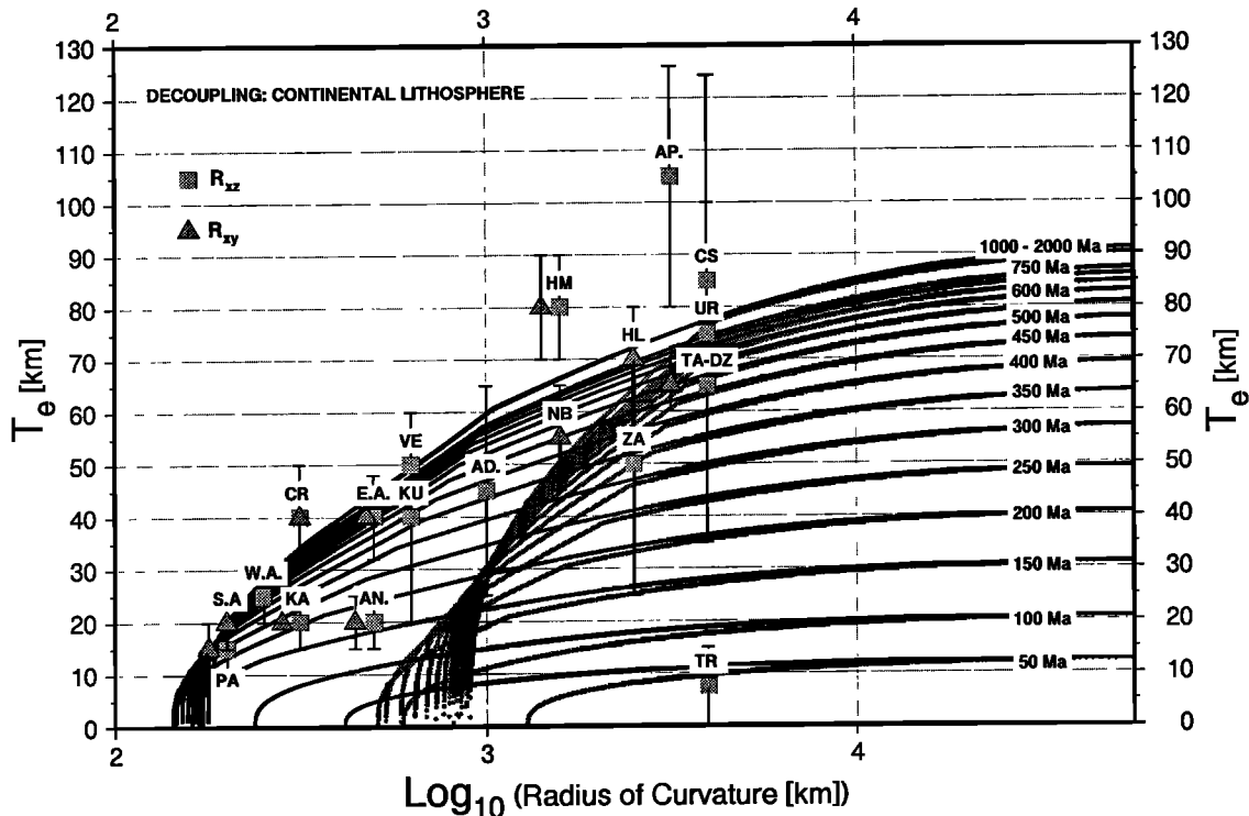
Figure 7b. Decoupled lithosphere (lower crust with low temperature of creep activation and/or young plates). The decoupled model fits most of the continental data except few cases where the lithosphere is likely to be coupled (Himalaya, Appalachians). The lithospheric flexure can dramatically decrease (by a factor of 3 or even 5, e.g., Pamir) the effective elastic thickness of the lithosphere. The coupled rheology (Figure 7a) cannot explain low T_e values for young lithosphere, as well as it provides worse fit to most middle-aged plates. One can also see that due to decoupling for equal ages the oceanic lithosphere may be even stronger than the continental lithosphere. The data sources on R_{xz} , R_{xy} for the continental lithosphere are R_{xz} (solid squares) McNutt et al. [1988]; The values of R_{xy} (solid triangles) are deduced from the geometries of plate deflection from Royden [1993], Burov et al. [1990], Burov and Diament [1992], Burov et al. [1994], Kruse and Royden [1994].
