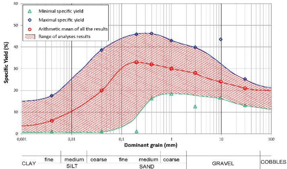
Figure 4. Range and arithmetic mean of specific yield values for 586 analyses in the Hydrol. Lab. of the US Geol. Survey (from Morris and Johnson, 1967).
