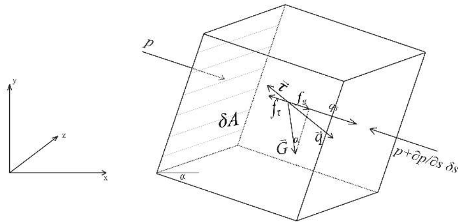
Figure 2. Definition sketch of liquid driving and opposed viscous forces for elemental volume.
