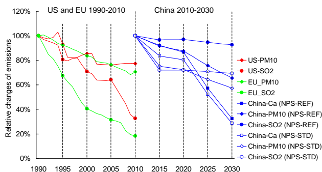
Figure 6. Relative changes of PM 10 and SO 2 emissions for the US (red) and EU (green) in 1990–2010 and those of PM 10 , Ca, and SO 2 for China in 2010–2030 under the NPS-REF (solid blue) and NPS-STD (hollow blue) scenarios in this work.
