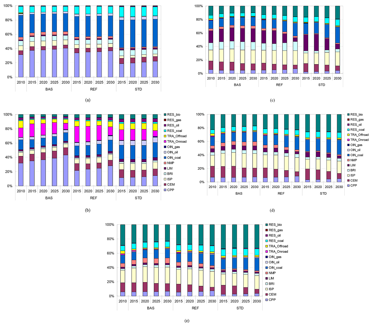
Figure 3. Shares of China's anthropogenic emissions by source for 2015, 2020, 2025 and 2030. Values are for the NPS activity scenario and three emission control levels: BAS, REF, and STD. (a) SO 2 ; (b) NO x ; (c) PM; (d) PM 10 ; and (e) PM 2.5 .
