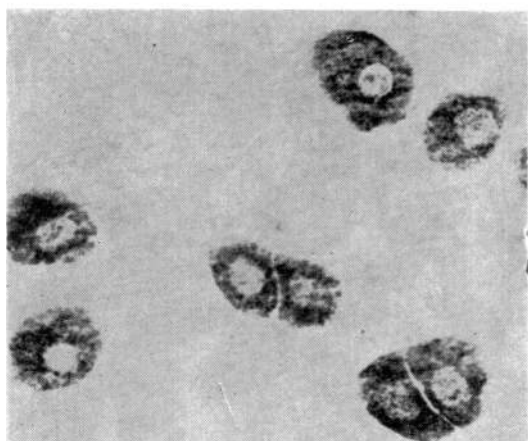
FIG. 2.—Subcutaneous tissue spreads from untreated rats in (a), and from rats treated for three days with intraperitoneal injections of 48/80 (doses as in text) (b), and reserpine 3 mg./kg. daily in (c). The spreads were stained with toluidine blue. Magnification, \times 680 .
