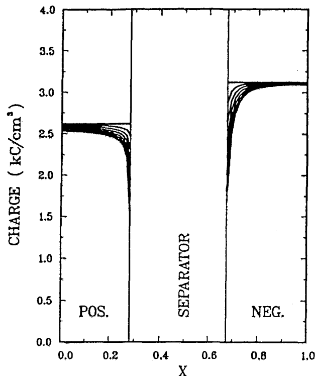
Fig. 6. State-of-charge profiles for 408 mA/cm 2 discharge at -18°C. Profiles from top to bottom are at time steps of 0, 5, 10, 15, 20, and 30s, respectively.
