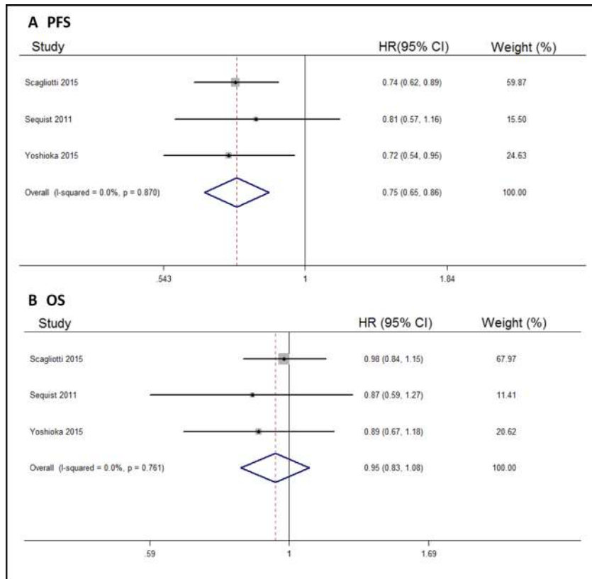
Figure 3: Forest plots of the pooled HRs for PFS and OS by NSCLC subgroup. (A) PFS, (B) OS.
