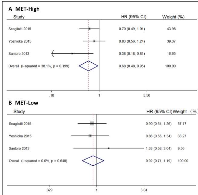
Figure 4: Forest plots of the pooled HRs for OS by MET status subgroup. (A) MET high subgroup, (B) MET low subgroup.
