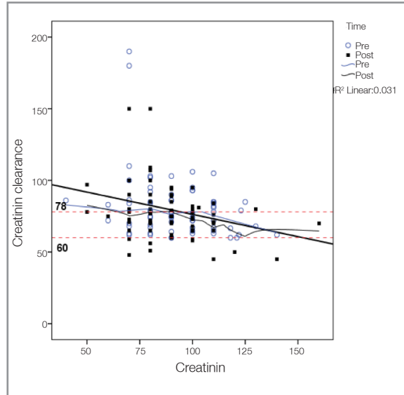
Figure 3. The scatter plot demonstrating the inverse linear relation between Cr and creatinine clearance value.
