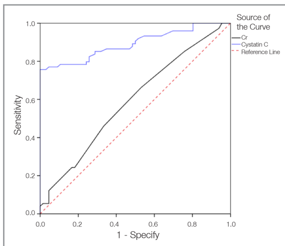
Figure 4. ROC Curve
