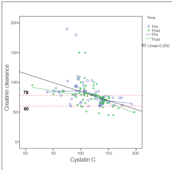
Figure 2. The scatter plot demonstrating the inverse linear relation between cystatin C and creatinine clearance value. However this relation was weak ( r=-0.447 , p<0.001 ).
