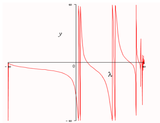
Figure 2 All eigenvalues in R
