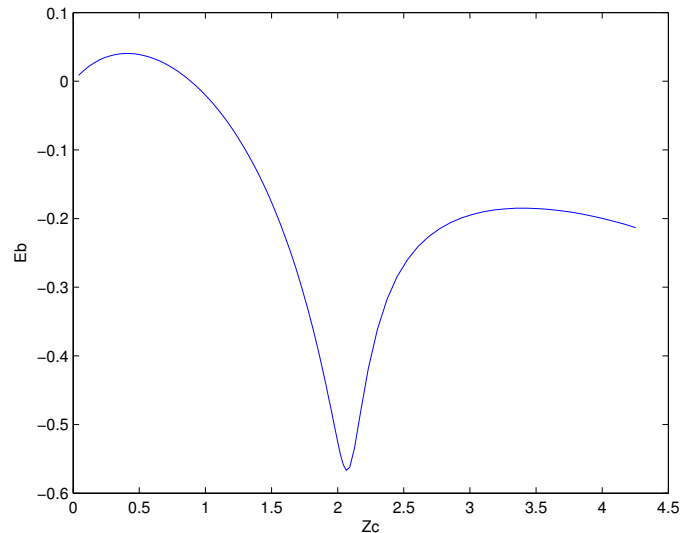
Figure 6: k = 0 , l = 3/2 , L_0 = 0.1
