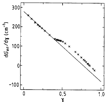
Figure 4. The derivative of the interaction part of the free enthalpy dG_{\text{int}}/d\gamma = \Delta - 2\gamma\Gamma of the compound [\text{Fe}(\text{2-pic})_3]\text{Cl}_2 \cdot \text{EtOH} versus the HS fraction \gamma . The step in the transition curve \gamma(T) gives rise to shift of the derivative in the transition region. The slope below and above the step is the same and determines the interaction constant to be \Gamma = 175 \text{ cm}^{-1} .
