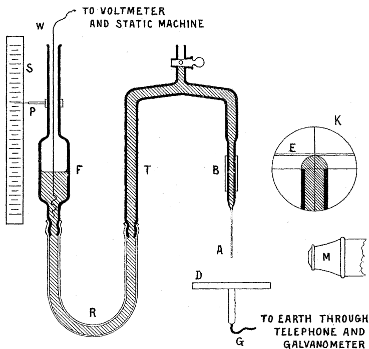
Fig. 1. Diagram of apparatus.
