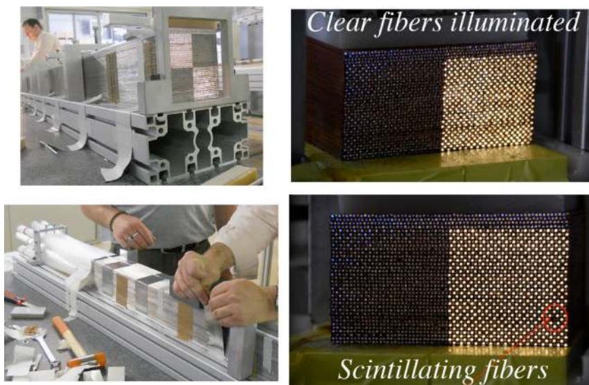
Fig. 2. Pictures of the first SuperDREAM modules built with lead (left) or copper (right) as absorber material. The alternating arrangement of clear and scintillating fibers in each row of the copper modules is illustrated by illuminating the fiber bunches from the rear end.
