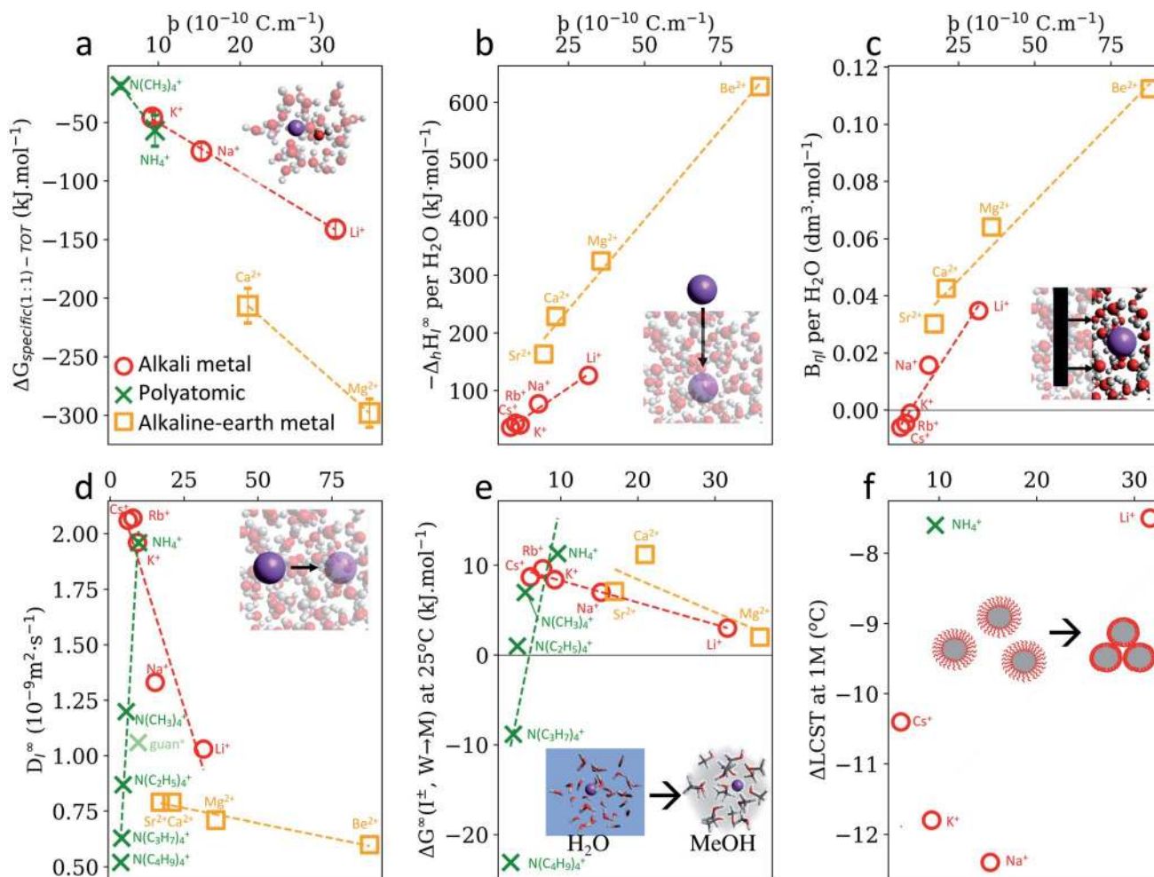
Fig. 4 SIE trends for cations do not always arise from cation–solvent Coulombic interaction, as measured by the descriptor \beta . (a) Specific ion–water interactions calculated from first-principles. (b) Experimental enthalpies of hydration per coordinating water molecule. 59 (c) Viscosity B-coefficients 59 of electrolyte solutions per coordinating water molecule (see also Fig. S11b†). (d) Diffusion coefficients of ions in water. 59 Gibbs free energies of ion transfer from water to methanol. 59 (f) \Delta LCST of pNIPAM-coated silica particles in 1 M electrolyte solutions. 60 Monovalent alkali metal cations (red circles) include \text{Li}^+ , \text{Na}^+ , \text{K}^+ , \text{Rb}^+ and \text{Cs}^+ ; polyatomic cations include \text{NH}_4^+ , \text{N}(\text{CH}_3)_4^+ , \text{N}(\text{C}_2\text{H}_5)_4^+ , \text{N}(\text{C}_3\text{H}_7)_4^+ , \text{N}(\text{C}_4\text{H}_9)_4^+ (green cross) and guanidinium + (light green cross); monatomic divalent alkaline earth metals include \text{Be}^{2+} , \text{Mg}^{2+} , \text{Ca}^{2+} , \text{Sr}^{2+} , \text{Ba}^{2+} (orange squares) and each set of data displayed has a common (or no) anion. U_E version in Fig. S31.† A full list of cation \beta values is provided in Table S31.†
