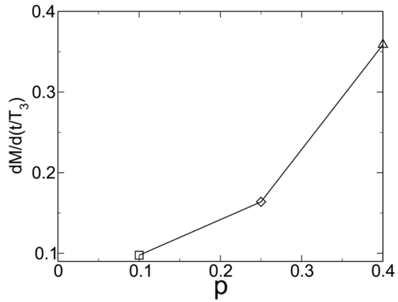
Figure 8. The rate of change of modularity increases with increasing magnitude of environmental change. From [38].
