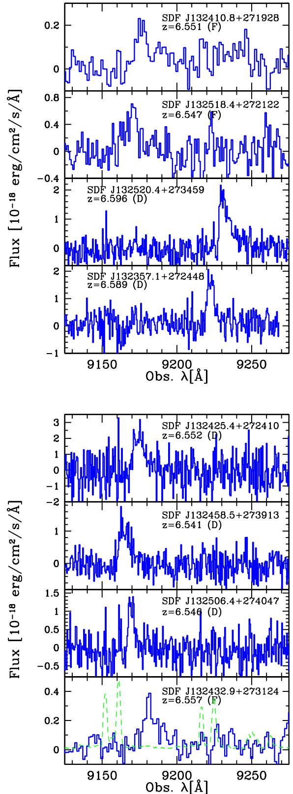
FIG. 1.— Spectra of eight spectroscopically confirmed z6p5LAEs. “F” (“D”) in parentheses indicates that the object was observed with FOCAS (DEIMOS). The sky spectrum is overlotted on the bottom panel with an arbitrary flux scale. The spectrum of SDF J132518.4+272122 which was identified as a LAE in this study already appeared in T05.
