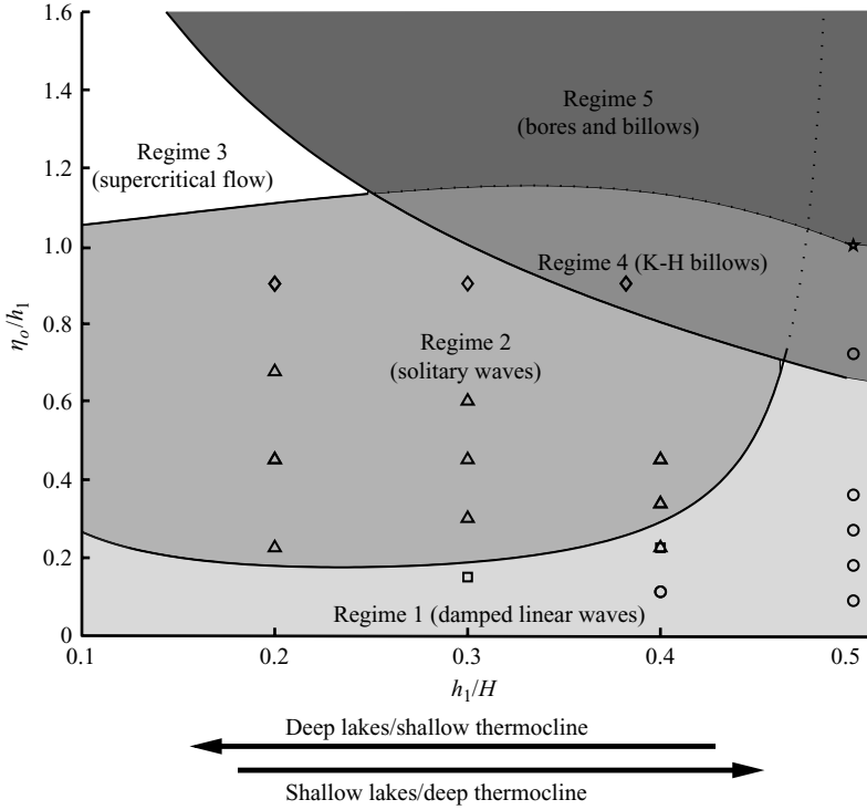
FIGURE 1. Analytical regime diagram characterizing the degeneration of large-scale gravity waves, plotted in terms of the normalized initial forcing scale \eta_0/h_1 and the depth ratio h_1/H . The laboratory observations are also plotted ( \star , Kelvin–Helmholtz (K-H) billows and bore; \diamond , broken undular bore; \triangle , solitary waves; \square , steepening; \circ , damped linear waves). Reproduced from Horn et al. (2001).
