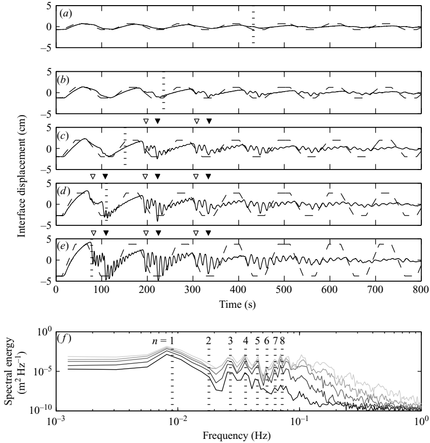
FIGURE 5. Time series of the observed interface displacement (solid line) and linear initial-value problem (broken line) at wave gauge C: (a) \eta_0/h_1=0.15 ; (b) \eta_0/h_1=0.27 ; (c) \eta_0/h_1=0.43 ; (d) \eta_0/h_1=0.59 ; (e) \eta_0/h_1=0.83 . For the time series shown h_1/H=0.3 , T_i=109 s and the vertical dotted lines denote T_s from equation (2.15). The \nabla and \nabla symbols denote crests of the observed H1 seiche and progressive surge, respectively. (f) Interface displacement spectra for the observed time series in (a) to (e). The bottom line corresponds to (a), etc. and the vertical dotted lines denote the frequencies of the lowest eight basin-scale standing modes calculated from (2.4).
