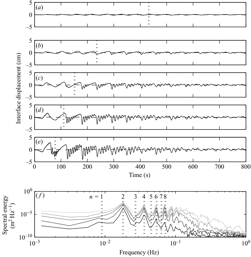
FIGURE 6. Same as figure 5 except at wave gauge B.
