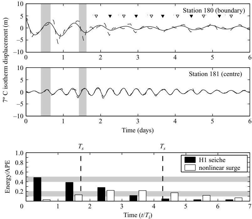
FIGURE 11. Raw (—) and filtered (---) time series of the 7^\circ isotherm displacement from Baldeggersee at (a) station 180 and (b) station 181. The time series are filtered as described in §3.3. The lake was subject to three along axis wind events. The first wind event ceases at the origin of the time axis, while the timing of the second and third events is denoted by vertical shading. The initial energy APE was evaluated as the maximum isotherm displacement, extrapolated to the lake perimeter, during the forcing events. The ▼ and ▽ symbols denote crests of the H1 seiche and progressive surge, respectively. (c) Temporal evolution of the APE distribution between the H1 seiche and progressive surge. Horizontal shading denotes the expected energy distributions as given by figure 8(a, e). For this data h_1 = 10 m (Lemmin 1987), H = 34 m (Imboden et al. 1983), \eta_0 \approx 5 m, W^{-1} = 0.4 , h_1/H = 0.3 , T_i \approx 16 h and T_s \approx 30 h. Note that in (c), T_s (---) is presented from the end of both the first and third wind events.
