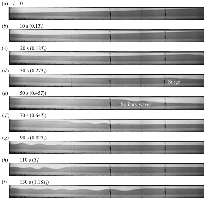
FIGURE 4. Video frames showing the standing seiche, evolving progressive surge and solitary waves. The initial condition is shown in (a). The surge and solitary wave packet are propagating to the left in (b)–(f), reflecting off the endwall in (g) and to the right in (h)–(i). For this experiment h_1/H = 0.3 , \eta_o/h_1 = 0.9 , T_i = 110 s and T_s = 40 s.
