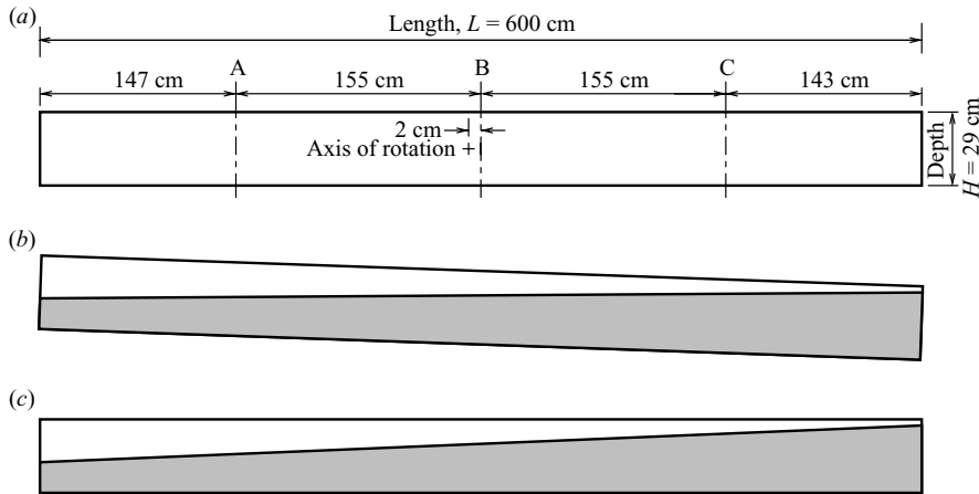
FIGURE 3. (a) Schematic diagram of the experimental set-up. The ultrasonic wave gauges were located at the positions marked A, B and C. (b) Initially tilted tank. (c) Initial condition with the tank horizontal and the interface inclined. Reproduced from Horn et al. (2001).
