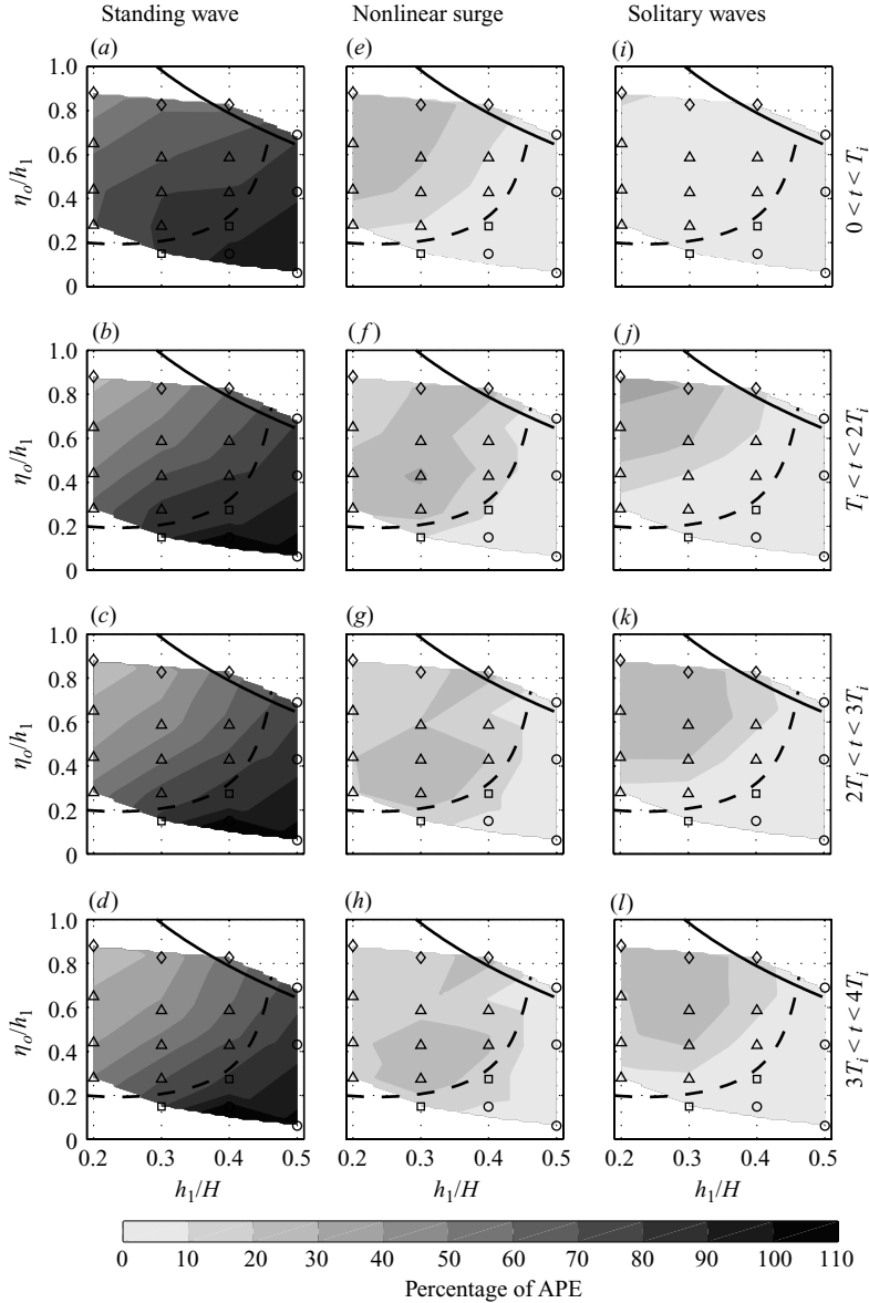
FIGURE 9. Same as figure 8, but viscous energy losses are accumulated with time along each column.
