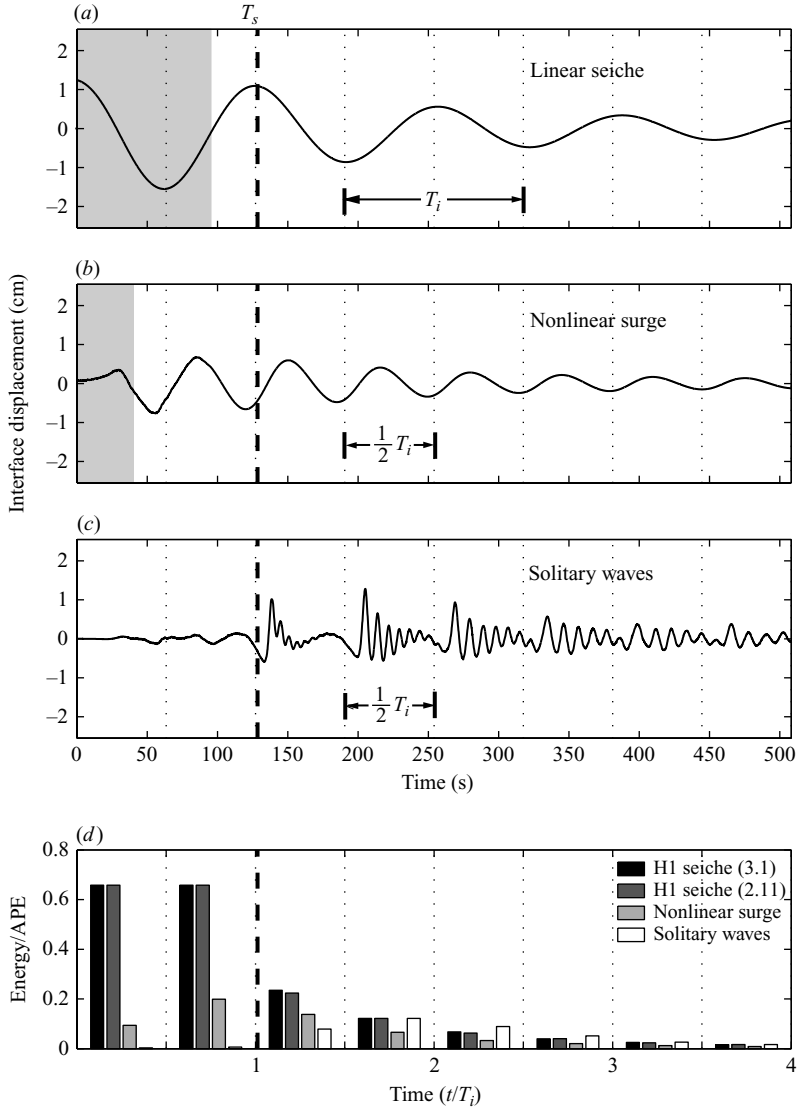
FIGURE 7. Filtered time series of the interface displacement for the experiment where W^{-1} = 0.44 and h_1/H = 0.2 . (a) Linear-seiche from low-pass filter ( f < (3/2T_i) ) of wave gauge A signal, (b) progressive surge from band-pass filter ( (3/2T_i) < f < (1/3T_i) ) of wave gauge B signal, (c) solitary waves from high-pass filter ( f > (1/3T_i) ) of signal of wave gauge B signal. Shaded region denotes region where transient filter start-up effects were corrected. (d) Temporal evolution of the APE distribution between the wave groups in (a)–(c).
