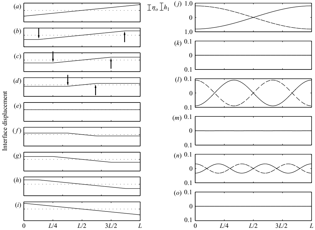
FIGURE 2. Solution of the wave equation initial-value problem resulting from a tilted interface. (a–i) Evolution of the interface position. Panels are shown over half an internal wave period ( 0 < t < T_i/2 ) at intervals of T_i/16 . The flow reverses (i.e. (i–a)) over T_i/2 < t < T_i . (j–o) Interfacial displacement of horizontal modes n=1 to 6, respectively, at t=0 (solid line) and t=T_i/2 (broken line). For description of arrows see text.
