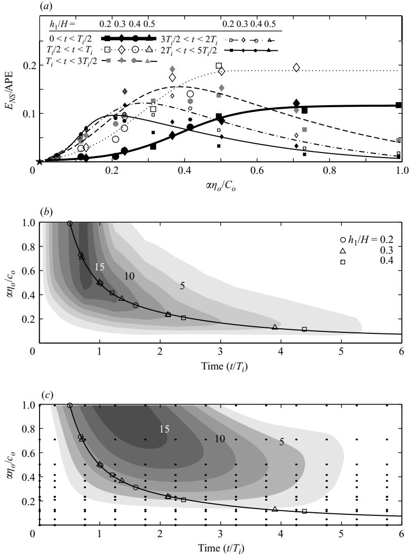
FIGURE 10. (a) Relationship between the fraction of APE observed as energy in the progressive surge E_{NS} , and the nonlinearity of the system \alpha\eta_0/c_0 over each of the first five T_i . Squares, diamonds, circles and triangles represent h_1/H = 0.2, 0.3, 0.4 and 0.5 , respectively. All curves are nonlinear least-squares fit. (b) Evolution of E_{NS}/APE in the (\alpha\eta_0/c_0, T_i) -plane from (a). (c) Evolution of E_{ISW}/APE in the (\alpha\eta_0/c_0, T_i) -plane. Contours are least-squares fit to the data points (indicated by \cdot ). In (a) and (b) the contours are presented as a percentage of the APE introduced at t = 0 with a contour interval of 2.5%. The solid line denotes T_i fitted to pass through values at h_1/H = 0.2, 0.3, 0.4 and 0.5 .
