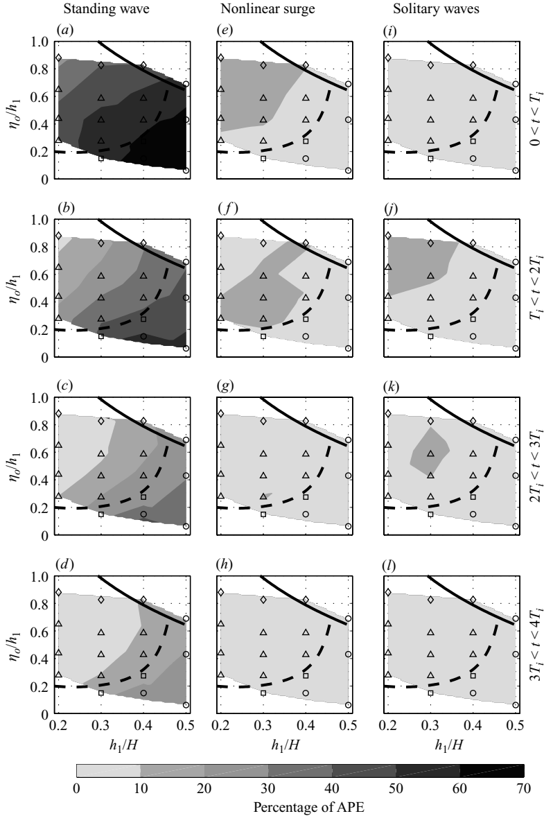
FIGURE 8. Temporal evolution of APE distribution between the component internal wave modes. The axes and regime boundaries of each panel are as in figure 1.
