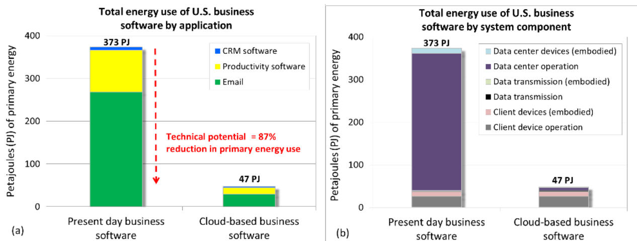
Figure ES-1: Primary energy use of present-day and cloud-based business software systems by: (a) application and (b) system component.
