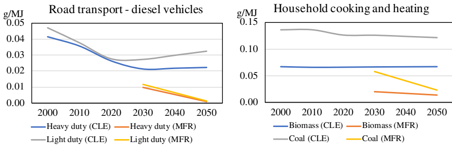
Fig. 1 Evolution of the baseline (CLE) and mitigation (MFR) case black carbon emission factors (at a global level) in the GAINS ECLIPSE V5a scenarios for two key sectors addressed in the BCOE-EndU scenario
