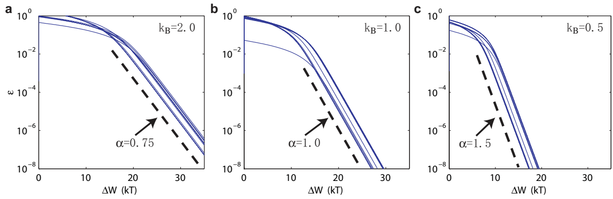
Figure S1: The dependence of \alpha on the k_B/k_R ratio. k_R = 1 is set to be unit to set the time scale. The \epsilon - \Delta W curves are computed for three different choices of k_B : a. k_B = 2.0 ; b. k_B = 1.0 ; c. k_B = 0.5 . \alpha can be determined by the slope of the semi-log plot, its values are 0.75, 1.0, 1.5 for the three cases shown here, and they agree with the expression \alpha = (1 + k_R/k_B)/2 .
