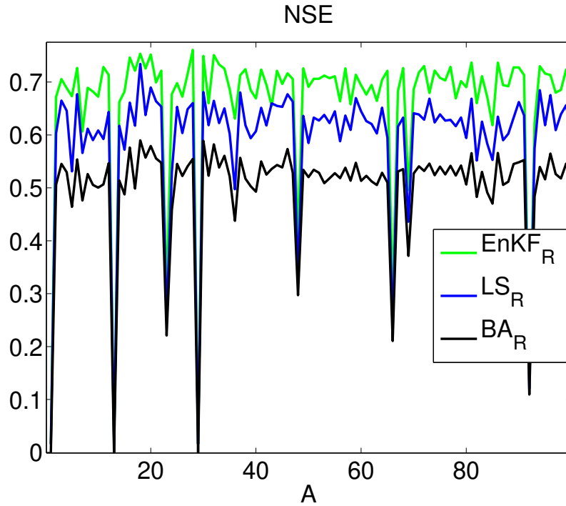
Figure 7. Comparison over an ensemble of random ensembles \mathcal{A} of the relative errors of one iteration of \text{EnKF}_R versus least squares ( \text{LS}_R ) and the best approximation ( \text{BA}_R ).
