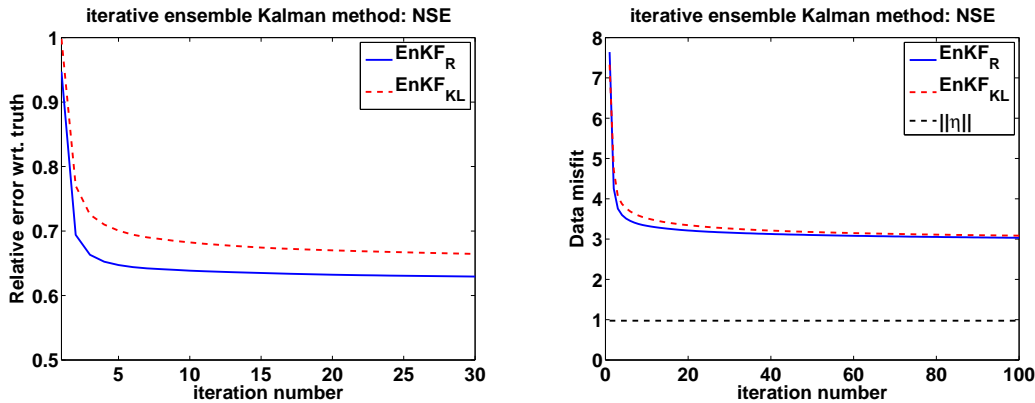
Figure 6. Performance of \text{EnKF}_R and \text{EnKF}_{KL} . Left: Relative error with respect to the truth. Right: Data misfit.
