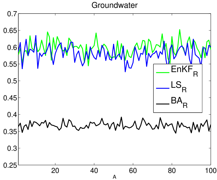
Figure 4. Comparison over different subspaces \mathcal{A} , generated from draws from the prior, of the relative errors of one iteration of \text{EnKF}_R versus (truncated iteration regularized) least squares ( \text{LS}_R ) and the best approximation ( \text{BA}_R ).
