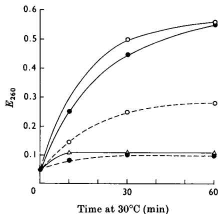
Fig. 1. Release of u.v.-absorbing compounds by ribonuclease from intact yeast cells (●), partly emptied cells (○) and cell wall fraction (△) with (---) or without (—) 10 mM-Mg 2+ . The incubation mixture contained 0.5 mg dry wt. of sample and 0.2 mg of ribonuclease/ml of water with or without 10 mM-Mg 2+ . After incubation at 30°C, the test samples were clarified by centrifugation, and the extinction at 260 nm was measured (cf. Alper, Dainko & Schlenk, 1967). The same curve (△) was obtained for cell walls with and without added Mg 2+ .
