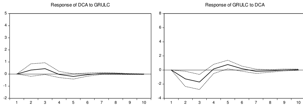
(a) Non-factorised innovations
