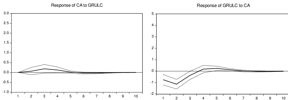
(c) Cholesky decomposition, only contemporaneous effects from CA to GRULC
