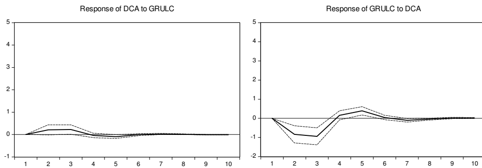
(a) Non-factorised innovations
