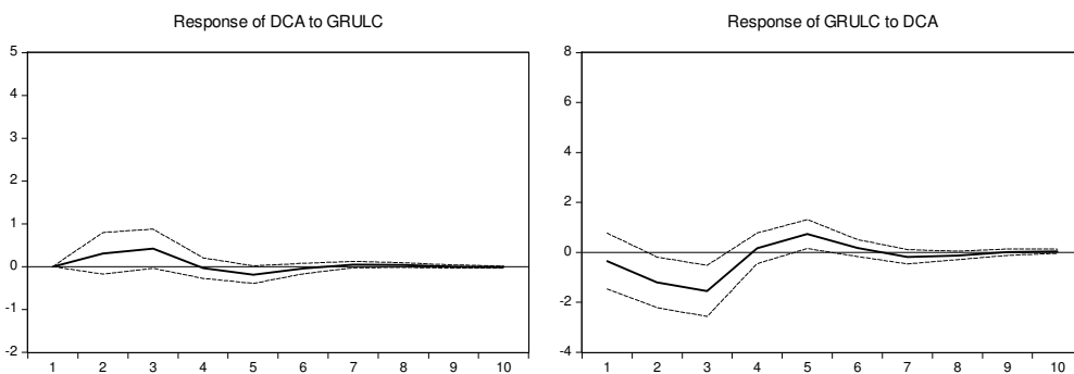
(c) Cholesky decomposition, only contemporaneous effects from DCA to GRULC
