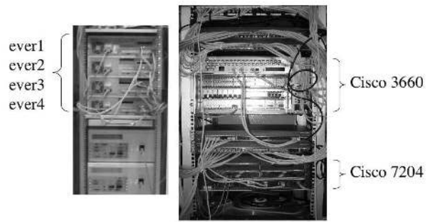
Figure 3. Testbed layout
