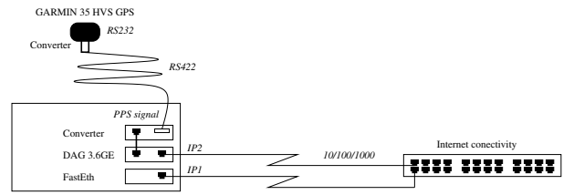
Figure 5. Monitoring node
