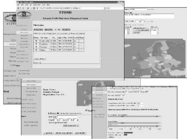
Figure 6. User interface
