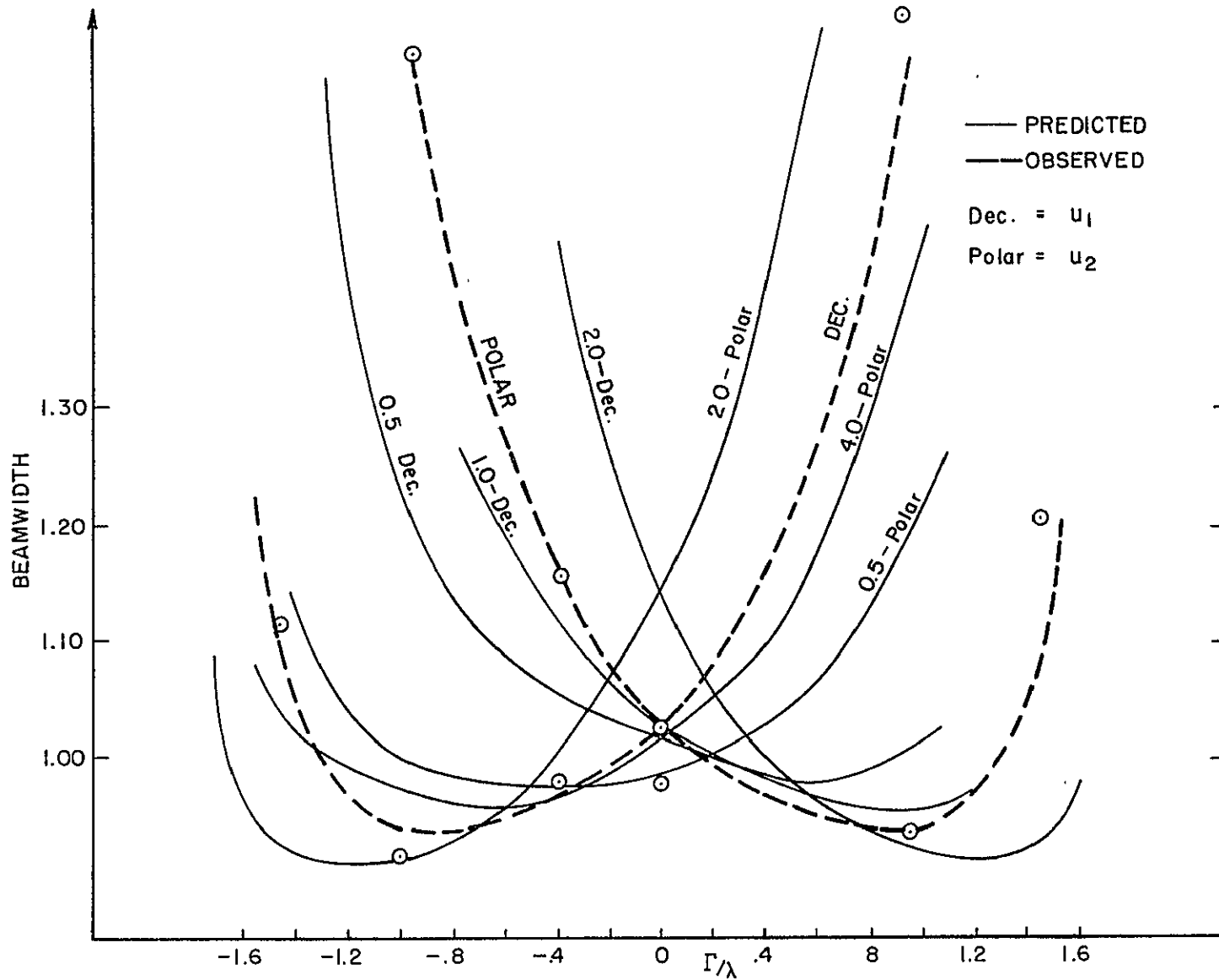
PREDICTION OF ASTIGMATISM WITH BEAM WIDTH MEASUREMENTS
