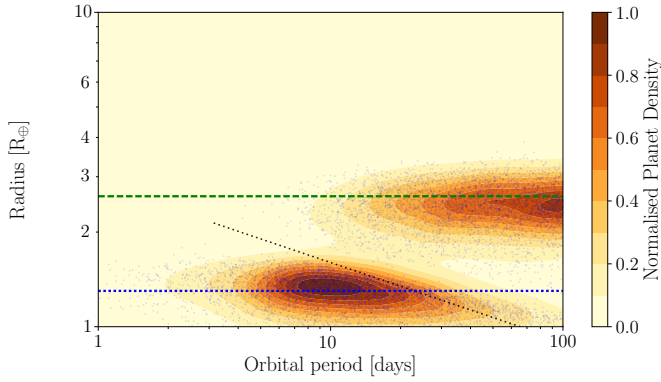
FIG. 9.— Similar to Fig. 5 but with an evaporation efficiency that is larger for less bound envelopes. (eq. 31). In this case, light planets can be stripped out to larger orbital distances, producing an extended tail of small planets out to \sim 100 days. For comparison, the dotted black line is eq. (28), applicable for models with a constant \eta = 0.1 .
