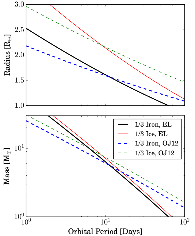
FIG. 10.— The position of the bottom of the evaporation valley (i.e. the largest stripped cores at a given period) shown in the top panel, with the core masses shown in the bottom panel. Solid lines show constant efficiency energy-limited models while dashed lines show evaporation models with variable efficiency similar to the Owen & Jackson (2012) evaporation models. The thick lines show Earth-like composition cores, while the thin lines shown those composed of 1/3 ice and 2/3 silicates.
