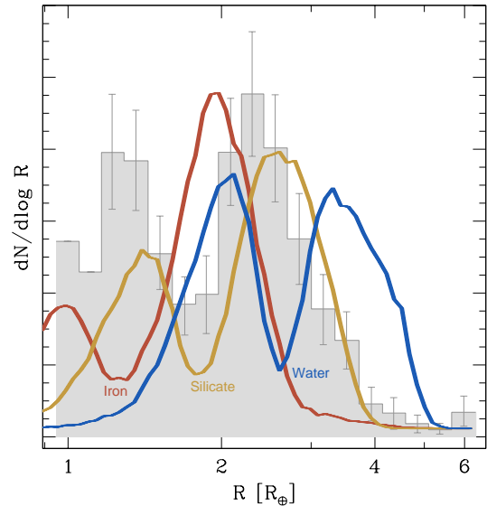
FIG. 7.— Comparing the valley location for cores made up of pure iron ( \rho_{M_{\oplus}} = 11 \text{ g cm}^{-3} ), pure silicate ( 4 \text{ g cm}^{-3} ) and pure water ( 1.3 \text{ g cm}^{-3} ). All parameters are otherwise identical, including the core mass distribution. The left-ward shifting of the valley with rising density is as prescribed in eq. (29). The observed data (grey shaded histogram) excludes ice-rich cores (blue curves) and favours compositions that are roughly terrestrial, namely, silicate-iron composite.
