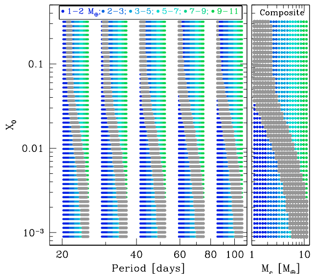
FIG. 3.— For a range of initial envelope mass fractions (y-axis), orbital periods (x-axis) and core masses (represented by different colors, slightly dispersed to the right for clarity), we calculate the final planet radius, at a few Gyrs, due to both cooling contraction and photoevaporation. Models are marked in grey if the final radii fall within the observed gap ( R = 1.8 \pm 0.2 R_{\oplus} ) and are thus disfavoured by the observations. The left panel shows the period dependence of these models, while the right panel shows the “composite” view: grey indicate any models that are excluded within the range of P = 20 - 100 days (the period range that the gap is clearly visible in data, Fulton et al. 2017). The initial planet population that can satisfy the observation fall into two categories: planets with masses more than two Earth masses and initial H/He masses more than a few percent; or lower mass planets with essentially no atmosphere. The star is assumed to be sun-like but the results are not particularly sensitive to the stellar mass.
