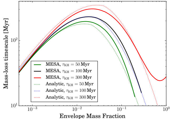
FIG. 1.— The timescale for envelope evaporation is plotted as a function of envelope mass fraction, from numerical models calculated with the MESA code (solid lines) and from our analytical model (eq. 20, dotted curves, smoothed as described in the text). The planet has a core mass of 5M_{\oplus} , an Earth-like core composition, and lies at a period of 10 days around a “Sun-like” star. See text for our choice of other parameters. Three types of models with different cooling ages are plotted. The numerical model with the longest cooling age shows an uptick at large envelope mass, resulting from self-gravity of the envelope, which compresses the envelope, an effect we ignore in our analytical model. For models with shorter cooling ages, numerical models at these masses do not converge, as their radii typically exceed the planet’s Bondi radius.
