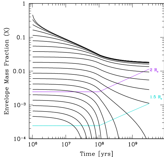
FIG. 2.— The erosion of atmosphere as a function of time, for planet models with a range of initial envelopes. All parameters are the same as in Fig. 1. As expected, almost all erosion occurs in the first 100 Myrs, when the planets are hot and when the stars are bright in high-energy radiation. Low mass envelopes are stripped clean, while higher mass ones are herded towards X \sim 1\% (and R_p \sim 2R_c ). The colored lines denote planet radii (values as marked, they differ from the estimate in eq. (17) because these are photospheric radius). This set of models resemble group (c) in Fig. 6.
