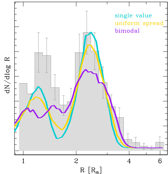
FIG. 8.— Same as Fig. 7, but now focussing on silicate-iron composites with different iron fractions ( f_{Fe} ). Different theoretical distributions correspond to models with: single value, f_{Fe} = 1/2 ; uniform spread, f_{Fe} \in [0, 1] ; bimodal, f_{Fe} = 0 or 1 . The data excludes the last distribution, but can not distinguish the first two. This illustrates our inability to constrain the iron fraction to a narrow range.
