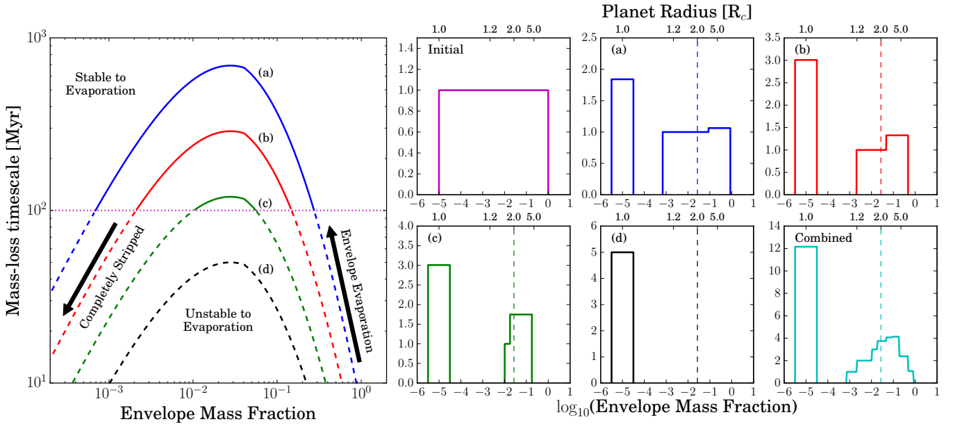
FIG. 6.— Schematic figures showing the mass-loss timescale (far left panel) and resultant envelope mass fraction histograms that result from envelope evaporation. The far left panel show the mass-loss timescale as a function of envelope mass fraction for four models – (a) through (d) – which are progressively closer and closer to their parent star. Those envelope mass fractions with mass-loss times < 100 Myr and unstable to evaporation and are shown as solid lines, whereas envelope mass fractions with mass-loss times > 100 Myr are stable to evaporation and are shown as dashed lines. The six small panels schematically shows what would happen to a population of planets. The top left small panel shows the initial envelope mass fraction distribution (arbitrary chosen to range between 10^{-5} and 1). The panels labelled (a) through (d) shows the resultant population due to evaporation. The bottom right panel shows the combination of models (a) through (d). The vertical dashed lines shows the envelope mass fraction which doubles the planet’s radius. We clearly see how evaporation generates a bimodal distribution in radius and envelope mass fraction.
