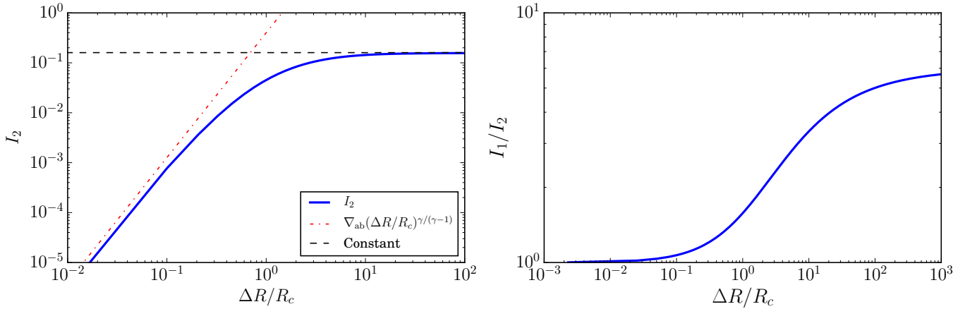
FIG. 11.— The numerical solutions of I_2 (left-panel) and I_1/I_2 (right-panel) are shown as the solid blue line. The approximations to I_2 used in the analysis in §2.1.1 in the limits \Delta R < 1 (red dot-dashed) and \Delta R > 1 (black dashed) are shown in the left-hand panel.
