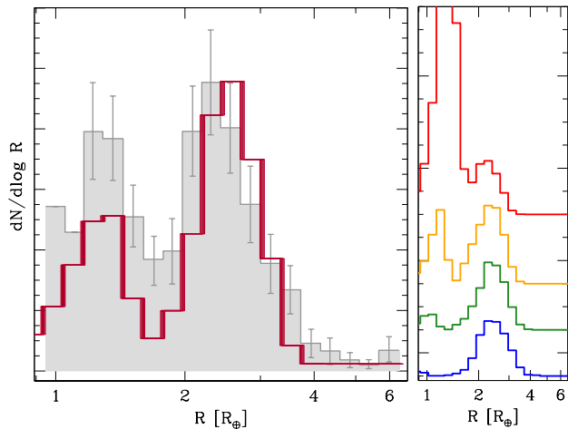
FIG. 4.— The final radius distribution after three billion years of evolution. The left panel shows the distribution for our entire model population (colored line). It compares well against the observed one from (Fulton et al. 2017), plotted here as shaded grey histogram, including the gap at 1.8R_{\oplus} , the peaks at 1.3R_{\oplus} and 2.6R_{\oplus} , as well as the sharp deficit of Neptune-like planets (size beyond 3R_{\oplus} ), note we did not attempt to “fit” the observed histogram (see text). The right panel displays the radius distribution binned by orbital periods. From top to bottom, the period bins are, 0 – 10, 10 – 20, 20 – 40, and 40 – 100 days.
