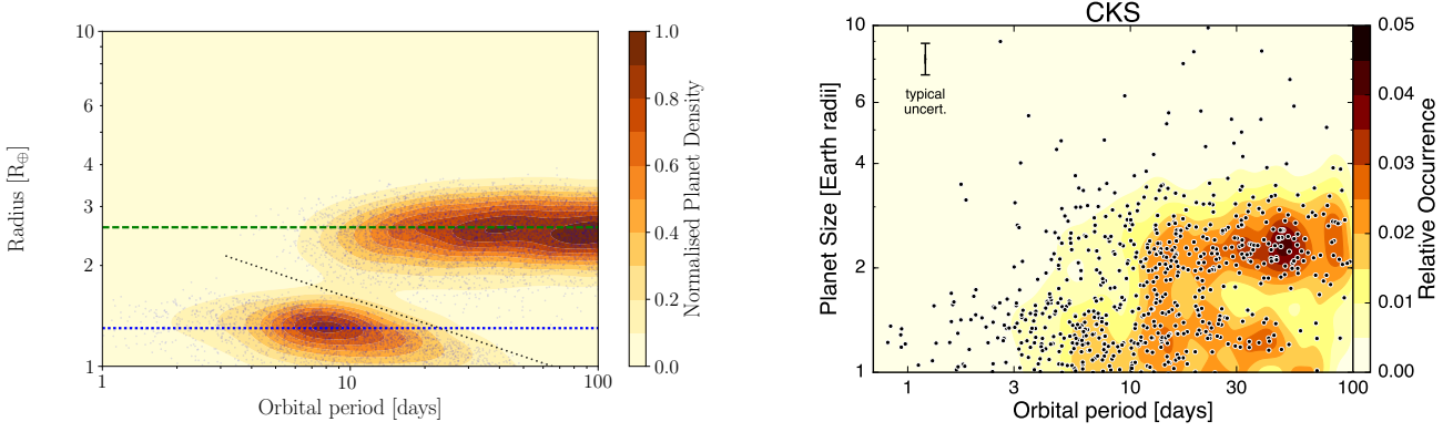
FIG. 5.— The final radius distribution, now plotted as 2-D contours to display the period dependence. The model largely reproduces the observed one (right side, taken from Fulton et al. 2017, with permission), with the exception of an absence of small planets at long periods in the model. The black dotted line is the analytical result (eq. 28) for the size of the most massive planet that can be stripped bare, at a given period. This marks the lower boundary of the “evaporation valley”.
