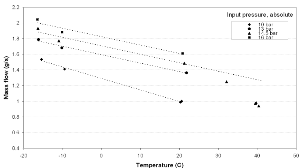
Figure 14. Mass flow as a function of liquid temperature before a capillary, measured for capillary with a nominal ID = 0.65 mm, and length of 2 m, with an evaporation pressure of 1.75 bar absolute with different input liquid pressures which are defined on the graph. The linear fits shown are performed for temperatures from 20 °C to −15 °C and are to guide the eye and illustrate the non-linear dependence of the massflow on liquid temperature.
