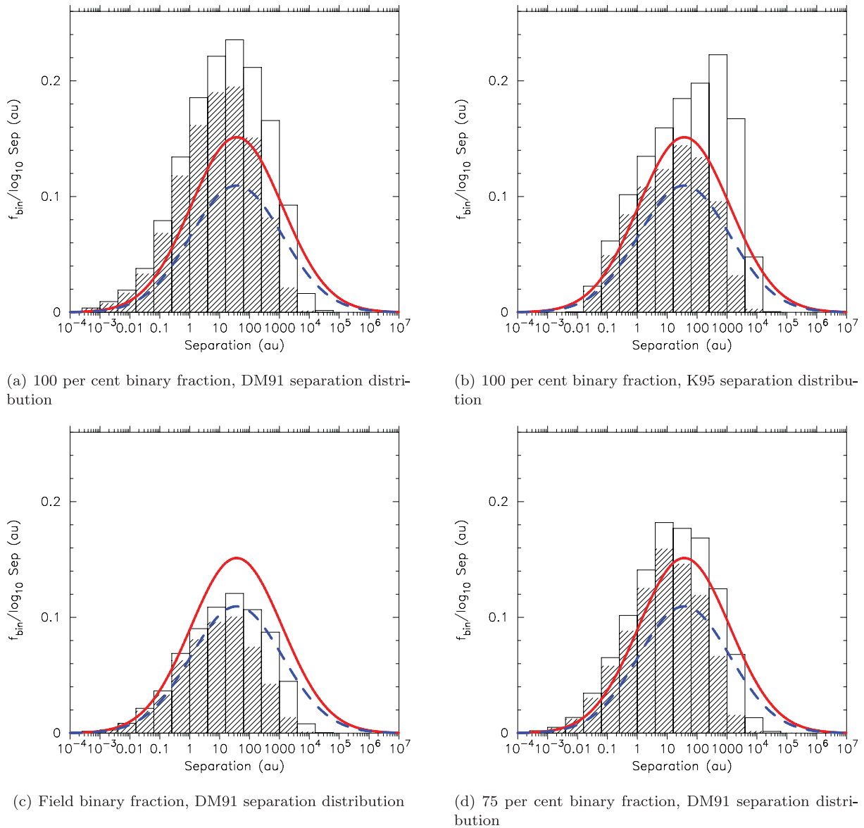
Figure 4. The full separation distributions at 0 Myr (open histograms) and 1 Myr (hashed histograms) for clusters with an initial fractal dimension D = 2.0 . Four different primordial binary population setups are presented, and the log normal fits to the separation distributions for G dwarfs and M dwarfs in the field [(red) solid and (blue) dashed lines, respectively] are shown for comparison.
