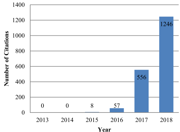
FIGURE 3. Yearly number of citations to blockchain papers.
