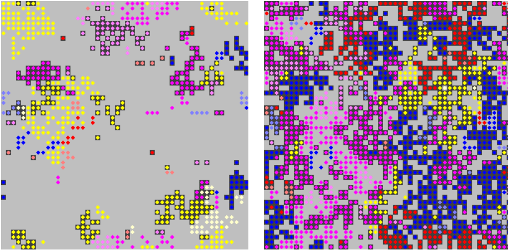
Figure 1. A typical run of the model after 100 periods (a) and 2000 periods (b). The shading of the foreground of a cell indicates the agent's strategy toward others of its own color, with a dark dot indicating cooperation. The shading of the background of a cell indicates the agent's strategy toward agents of other colors, with black indicating defection. Thus agents using the ethnocentric strategy have a dark dot on a black background, and egoist agents have a light dot on a black background. A movie of this run is available on the web in Quicktime format at: www.umich.edu/~axe/EXP104.mov
