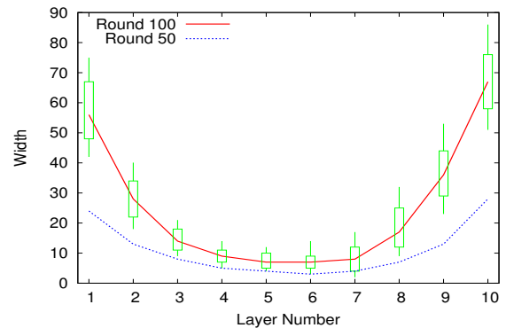
Figure 4: The median width of each layer at round-50 and round-100 (percentiles are only shown for the latter).
