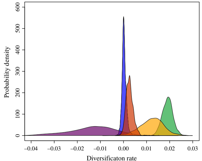
Fig. 4 Diversification rates for dormancy classes. Diversification rate (speciation – extinction rate) is given on the x-axis, and the probability density on the y-axis. Nondormancy (ND), blue; physiological dormancy (PD), green; morphological dormancy (MD), orange; morphophysiological dormancy (MPD), red; physical dormancy (PY), purple. Rate estimate distributions were aggregated from Markov chain Monte Carlo (MCMC) runs of the MuSSE model with 1 \times 10^3 iterations, with a 10% burn-in for each of 100 trees. Results are for the Dorm5B dataset. See Table S8 and Fig. S2 for additional results.
