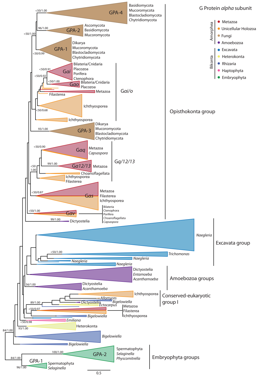
FIG. 4. —Maximum likelihood (ML) phylogenetic tree inferred by the G protein \alpha subunit. Different eukaryotic lineages are represented by a color code depicted in the legend. Within the gene family clades, the specific taxonomic groups which comprise eukaryotic lineages represented in that clade (i.e., eumetazoans and placozoans) are shown on the right. Nodal supports indicate 100-replicate ML bootstrap support and Bayesian posterior probability (BPP). Supports are only shown for nodes recovered by both ML and Bayesian inference, with BPP > 0.9.
