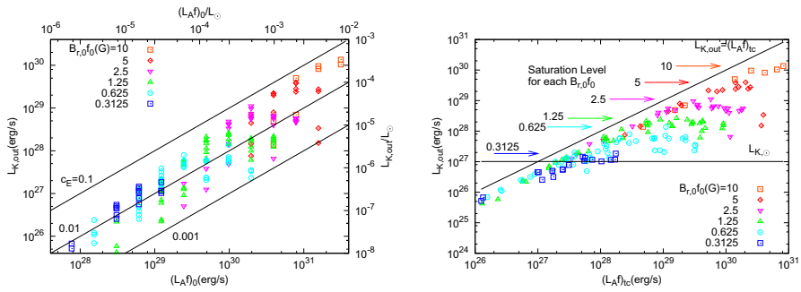
Fig. 19 Left: The output kinetic luminosity ( \dot{M}u_r^2/2 , y-axis) of stellar winds increases with the input wave luminosity (x-axis) at the photosphere (subscript ‘0’). Different values of magnetic field strengths are shown by the different symbols. Curves of constant ratios between y-axis and x-axis (labeled c_E ) are shown by the solid lines. Right: The same as the left panel, but instead of the input wave luminosity, the x-axis now shows the wave luminosity as measured at the transition region (top of the chromosphere, subscript ‘tc’). Images reproduced with permission from Suzuki et al. (2013), copyright by ASJ
