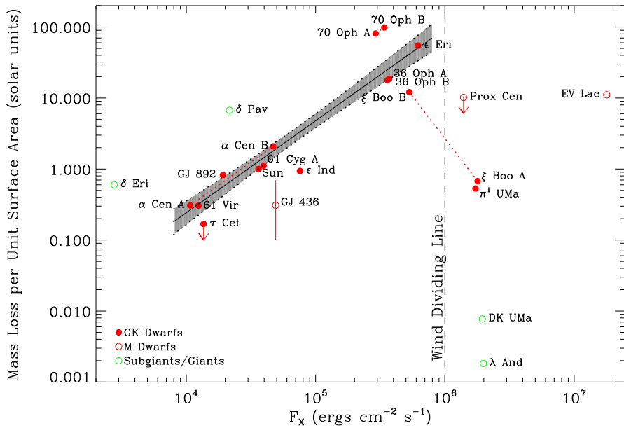
Fig. 4 Summary of mass-loss rates for low-mass stars derived from the astrosphere method. For GK dwarfs (red filled circles), the mass-loss rate per unit surface area varies as a function of X-ray flux as \propto F_X^{1.34} (shaded line). It has been suggested that active (and overall younger) stars with F_X \gtrsim 10^6 \text{ erg s}^{-1} \text{ cm}^{-2} would have reduced mass-loss rates, thus giving rise to a ‘wind dividing line’. Some new mass-loss rates measurements indicate that mass-loss rates of young Suns could actually remain large (cf. Sect. 3). Image reproduced with permission from Wood (2018), copyright by the author
