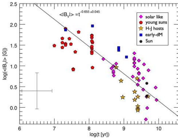
Fig. 14 The average unsigned large-scale magnetic field decays with age as t^{-0.655} . This is a similar trend as seen in \Omega_{\star}(t) (Eq. 22). Different symbols correspond to different ZDI surveys. Note that the Sun is represented at minimum and maximum phases of its magnetic cycle. Typical error bars are indicated on the bottom left. Image reproduced with permission from Vidotto et al. (2014a), copyright by the authors
