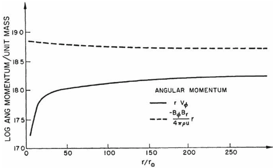
Fig. 24 The specific angular momentum of the solar wind calculated by Weber and Davis (1967). The sum of these two terms is constant with distance and simplifies to \mathcal{L} = \Omega_\star r_A^2 (see Eqs. 58 and 60), where r_A is the distance to the Alfvén point. Image reproduced with permission, copyright by AAS
