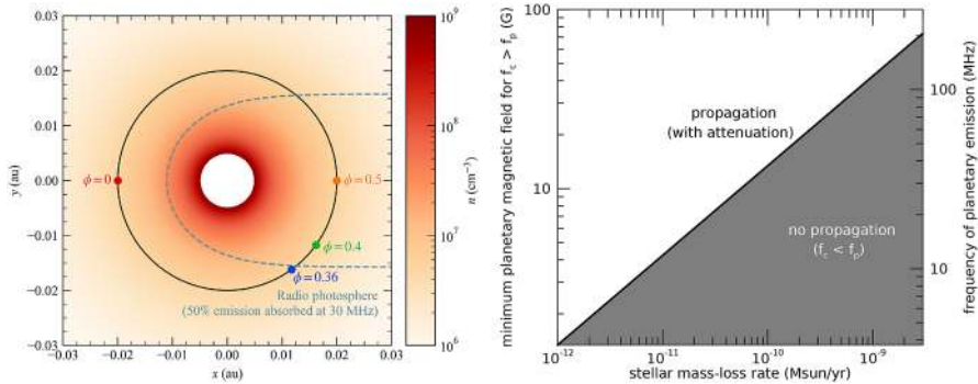
Fig. 7 Left: Number density of the wind of a solar-like star with a mass-loss rate of 2 \times 10^{-12} M_{\odot} \text{yr}^{-1} . A planet is considered to orbit at 0.02 au, with the observer looking towards the system from the negative x -direction. The dashed line shows the radio photosphere where 50% of a 30-MHz wind emission is produced. The hypothetical 30-MHz radio emission of this planet is increasingly more attenuated after the planet ingresses the radio photosphere and the attenuation peaks at orbital phase \phi = 0.5 . Its emission is least attenuated at \phi = 0 . Given that the position of the radio photosphere is linked to the stellar wind properties, monitoring of planetary radio emission could allow one to derive stellar wind properties. Right: The situation on the left panel only occurs if the plasma emission f_p is below the cyclotron frequency f_c of the planetary emission (white area). If the wind of the host star has a high mass-loss rate and the planet has a weak magnetic field, such that f_p > f_c , then the planetary radio emission cannot propagate through the wind of the host star (grey area). Detections of planetary radio emission can thus place an upper limit on the mass-loss rate of the star (Eq. 8). Note that the wind parameters used to produce this figure is based on models of the weak-lined T Tauri star V830 Tau. Images reproduced with permission from [left] Kavanagh and Vidotto (2020), copyright by the authors; and from [right] Vidotto and Donati (2017), copyright by ESO
