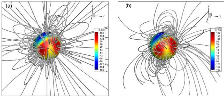
Fig. 20 a Magnetic field line extrapolations, assuming a potential field source surface model. The surface magnetic field is derived from ZDI observations (Donati et al. 2008). The potential field model assumes the stellar magnetic field is in its minimum energy state. b The field lines are stressed after interaction with stellar wind flow. Based on the simulations presented in Vidotto et al. (2014b)
