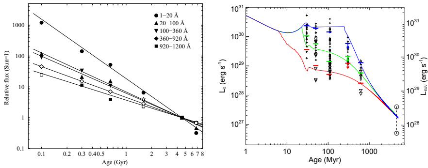
Fig. 17 Evolution of high-energy irradiation of solar type stars. Left: The observed evolution of high-energy flux at a given orbital distance at different bands. Right: The X-ray (left axis) and extreme ultraviolet (right axis) luminosities derived from rotational evolution tracks (e.g., Fig. 15) as a function of stellar age. Images reproduced with permission from (left) Ribas et al. (2005), copyright by AAS; and (right) Tu et al. (2015), copyright by ESO
