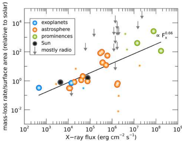
Fig. 8 Summary of derived mass-loss rates for low-mass stars combining results from the different methods discussed in Sect. 2. The y-axis is given in solar values, i.e., \dot{M}_\star/R_\star^2 , with \dot{M}_\odot = 2 \times 10^{-14} M_\odot \text{yr}^{-1} . Colour indicates the method used in the derivation: blue for exoplanets, orange for astrospheres, green for prominences, black for the Sun at minimum/maximum of its sunspot cycle. Grey arrows indicate upper limits, which are mostly derived from radio observations. The solid line is a power-law fit through the larger circles. The smaller symbols are either evolved stars or M dwarfs, which were not included in the fit and neither were the stars for which only upper limits exist (arrows). The values used in this plot were compiled from the following works: Drake et al. (1993); Lim et al. (1996); Gaidos et al. (2000); Wood et al. (2001, 2002, 2005a, 2014); Wood and Linsky (2010); Wood (2018); Wargelin and Drake (2002); Bourrier et al. (2013); Kislyakova et al. (2014); Fichtinger et al. (2017); Vidotto and Bourrier (2017); Vidotto and Donati (2017); Jardine and Collier Cameron (2019); Finley et al. (2019); Ó Fionnagáin et al. (2021)
