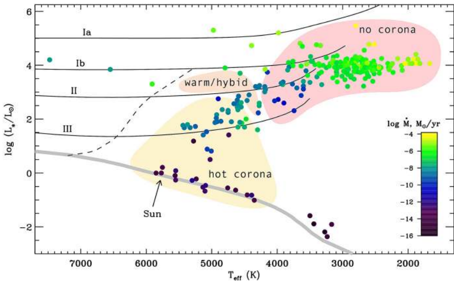
Fig. 2 An overview of mass-loss rates (colour coded) in the cool-star HR diagram. Winds of cool stars evolve from hot ( \sim 10^6 K) and tenuous ('hot corona') to cold ( \sim 10^4 K) and denser ('no corona'). Evolved low-mass stars that show weak or sporadic signatures of a hot corona are denoted 'warm/hybrid'. The zero-age main sequence is shown by the grey line. Image reproduced with permission from Cranmer and Winebarger (2019), copyright by Annual Reviews
