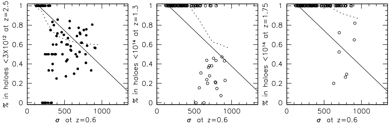
FIG. 15.—Clusters at high redshift. The solid line is the line drawn in the O \Pi - \sigma diagram observed at high redshift. Left: Filled circles represent the fraction of galaxies in 90 haloes selected at z = 0.6 in the MS simulation that were in haloes with mass < 3 \times 10^{12} M_{\odot} at z = 2.5 . The dashed line is the prediction of the average fraction of mass in haloes < 3 \times 10^{12} M_{\odot} at z = 2.5 derived from the PS formalism. Middle: Open circles represent the fraction of galaxies in the MS simulation that were in haloes with mass < 10^{14} M_{\odot} \sim 3 Gyr prior to z = 0.6 , thus at z = 1.3 . The dashed line is the prediction of the fraction of mass in haloes < 10^{14} M_{\odot} at z = 1.3 derived from the PS. Right: Open circles represent the fraction of galaxies in the MS simulation that were in haloes with mass < 10^{14} M_{\odot} \sim 3 Gyr prior to z = 0.8 , thus at z = 1.75 . The dashed line is the prediction of the fraction of mass in haloes < 10^{14} M_{\odot} at z = 1.75 derived from the PS.
