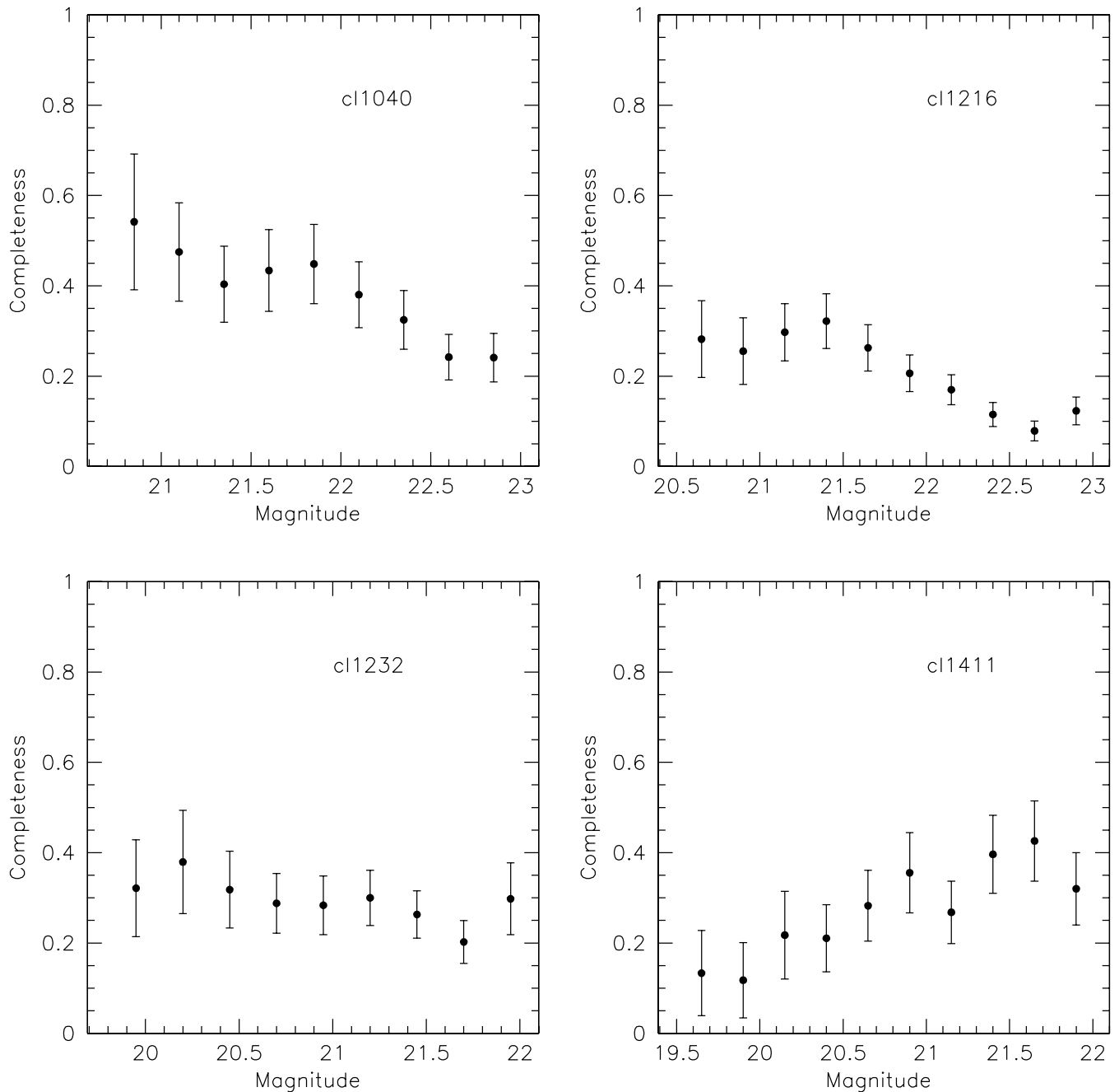
FIG. 17.—Completeness functions vs. galaxy magnitudes for four EDisCS clusters.
