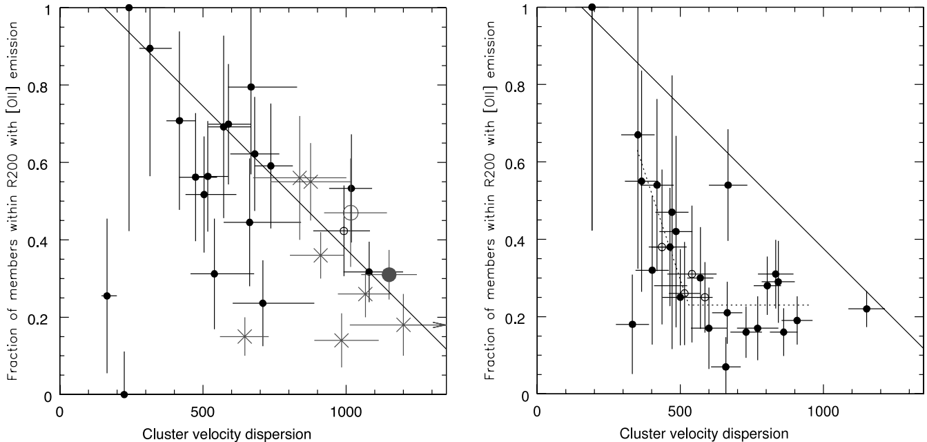
FIG. 4.— Left : O\ II-\sigma relation in clusters at 0.4 \leq z \leq 0.8 . The fraction of cluster members within R_{200} with O\ II emission is plotted vs. the cluster velocity dispersion. Filled circles represent EDisCS data points in each one of the 18 fields, as in Table 1. The crosses are for MORPHS clusters; the large filled circle is the cluster MS 1054–03 from van Dokkum et al. (2000), and the large open circle is CI 1324+3011 from Postman et al. (2001). Error bars on the fractions are Poissonian. The solid line across the plot is taken as a description of the upper envelope of the high- z points (see text). The same line is repeated in the right panel, to illustrate the differences. At high z , the majority of systems group around this line, while at low z ( right panel ) the great majority fall well below the line. Right : O\ II-\sigma relation in low-redshift clusters from SDSS described in § 4. Open circles indicate those SDSS clusters slightly outside of the preferred redshift range. The two dashed lines represent the eye-fitted most heavily populated region in the plot. [See the electronic edition of the Journal for a color version of the left panel of this figure.]
