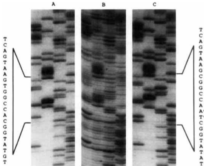
Fig. 2. Evidence for multiple alleles in the 18S rDNA sequence(s) obtained from A. pustulosa GE3a. B. Overlapping sequence obtained directly from the PCR products using primer 892c [11, 32]. A, C. Two different sequences obtained after cloning the PCR products. The sequences are located in stem 29.1 approximately at base 1321 in GE3a. The sequence reads in the 5' to 3' direction from the bottom to the top. The two sequences indicate the presence of two different alleles.
