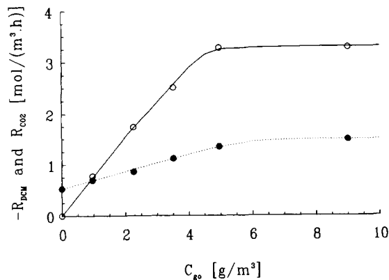
Figure 6. The DCM elimination (○) and simultaneous production of CO 2 (●) in the BTF vs. the inlet DCM concentration (performance curve) as determined at day 207.
