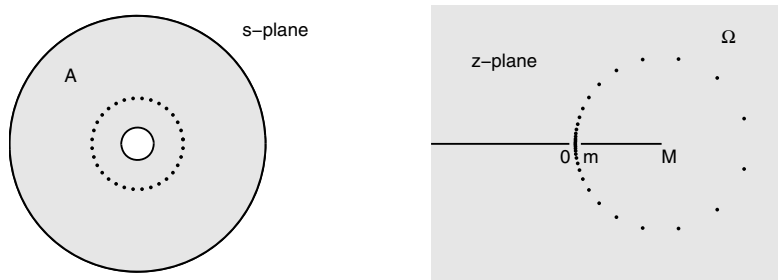
Fig. 18.2 By a conformal map to an annulus, the rate of convergence can be improved greatly to O((1 - (\log(\kappa))^{-1})^N) (figure from [71]).
