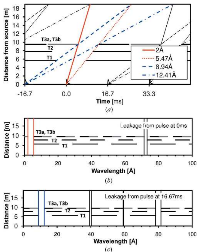
Figure 6 (a) Time diagram for the frame-skipping operation at 30 Hz with SDD = 19 m. Frames 1 from even-numbered pulses (at 0, 33.33 ms etc.) are allowed to pass through the choppers. At the same time, frames 3 from odd-numbered pulses (at -16.67, 16.67 ms etc.) are allowed to pass through as well. On the detector, these two frames do not overlap and can be treated separately. (b), (c) Neutron leakages through the choppers from even- and odd-numbered pulses, respectively.
