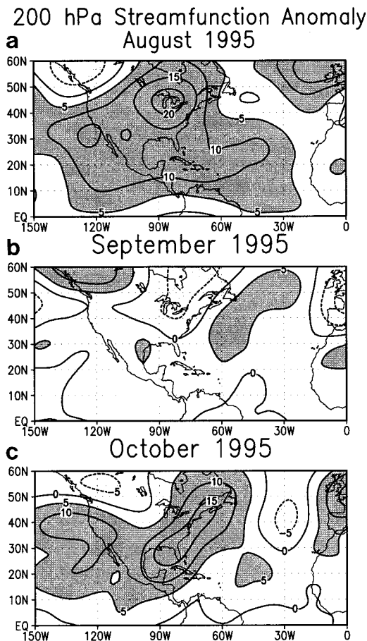
FIG. 14. The 200-mb streamfunction anomalies during (a) August, (b) September, and (c) October. The contour interval is 5 \times 10^6 \text{ m}^2 \text{ s}^{-1} , with positive (negative) values dashed (solid) and values greater (less) than 5 (-5) \times 10^6 \text{ m}^2 \text{ s}^{-1} shaded dark (light). The nondivergent component of the flow is directed along the streamfunction contours with a speed proportional to the gradient. Thus, high (low) streamfunction values correspond to high (low) geopotential heights. Anomalies are departures from the 1979–95 base period means.
