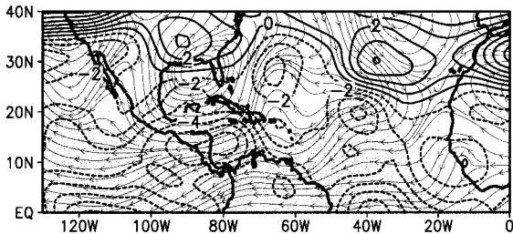
FIG. 4. August–October anomaly values of (a) the vertical shear magnitude [contour interval is 1.5 \text{ m s}^{-1} , with weaker (stronger) than average shear values dashed (solid) and shear that is at least 3 \text{ m s}^{-1} weaker than climatology is shaded]; (b) the vertical shear vector (contour interval is 2 \text{ m s}^{-1} , with values larger than 4 \text{ m s}^{-1} shaded); (c) the 200-mb streamlines and zonal wind speeds [contour interval is 2 \text{ m s}^{-1} , with positive (negative) values solid (dashed) and any easterly component greater than 2 \text{ m s}^{-1} is shaded]; and (d) the 850-mb streamlines and zonal wind speeds [contour interval is 2 \text{ m s}^{-1} , with positive (negative) values solid (dashed) and any westerly component greater than 2 \text{ m s}^{-1} is shaded]. Anomalies are departures from the 1979–95 base period monthly means.
