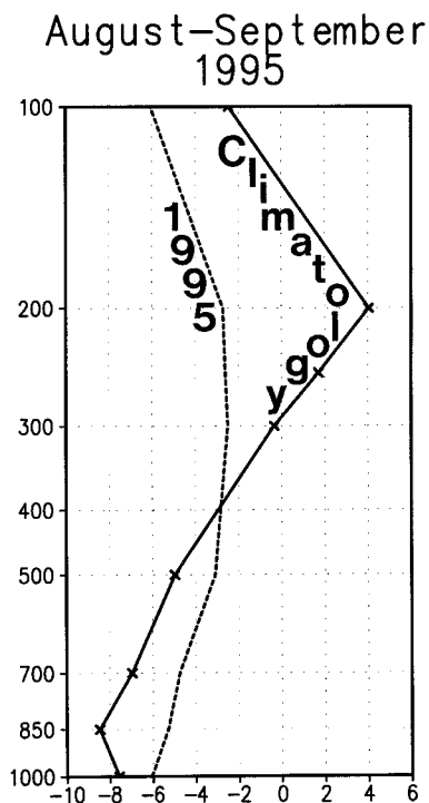
FIG. 5. August–September vertical profiles of the mean zonal wind for the Caribbean strip at 70°W along 10°–20°N for 1995 (dashed lines) and for the 1979–95 climatology (solid line).
