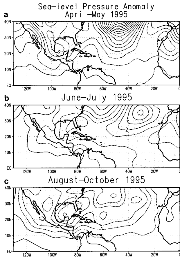
FIG. 7. SLP anomalies (mb) for (a) April–May 1995, (b) June–July 1995, and (c) August–October 1995. Contour interval is 0.5 mb, with positive (negative) values shown solid (dashed). Anomalies below -1.0 mb are shaded. Anomalies are departures from the 1979–95 base period monthly means.
