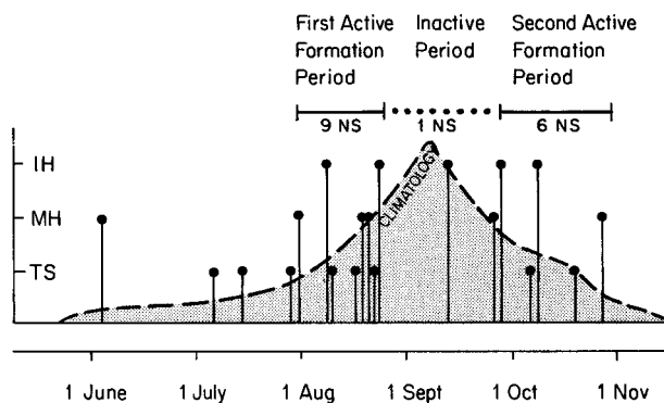
FIG. 13. Time line showing the dates when the 19 named storms of 1995 first attained tropical storm status. These storms tended to cluster during two active periods (30 July–29 August and 27 September–27 October). Note the relatively inactive period during 30 August–26 September that coincided with the normal climatological peak in activity.
