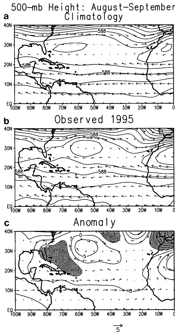
FIG. 16. August–September 500-mb heights and winds for (a) climatology (1979–95), (b) 1995 mean, and (c) 1995 anomaly. Contour interval for heights is 15 m and for height anomalies is 5 m. In panel (c), positive height anomalies are contoured solid and values greater than 5 m are shaded light. Negative height anomalies are contoured dashed and values less than -5 m are shaded dark.
