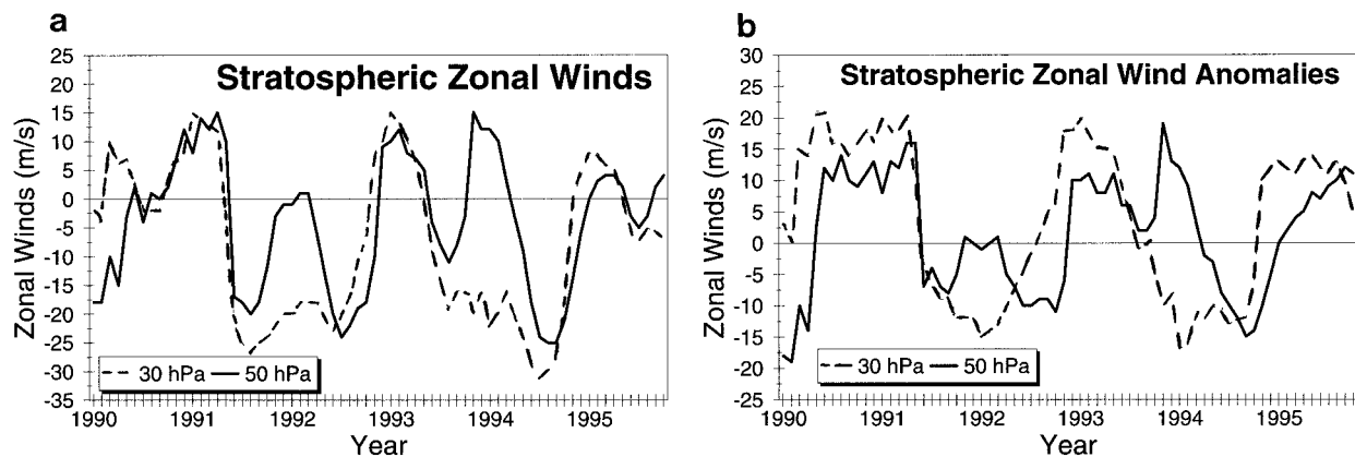
FIG. 10. Time series of (a) stratospheric zonal winds and (b) anomalies averaged between Curacao ( 12^{\circ}\text{N} ), Barbados [ 13^{\circ}\text{N} and Trinidad ( 11^{\circ}\text{N} )]. Values at 50 mb (30 mb) are shown by solid (dashed) curves. Units are meters per second. Anomalies are calculated from the 1950–90 base period monthly means.
