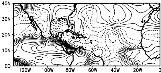
a Vertical Shear Magnitude
