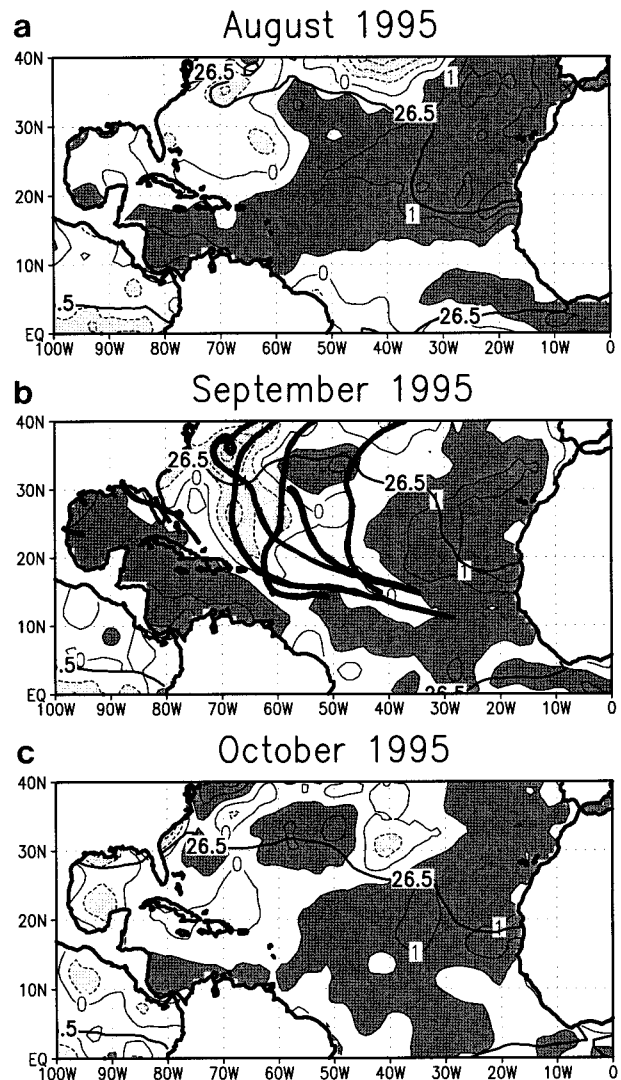
FIG. 15. Same as Fig. 8 except for (a) August, (b) September, and (c) October 1995 SSTs and SST anomalies. Solid lines in (b) indicate tracks of Atlantic tropical cyclones that formed from late July through late August.
