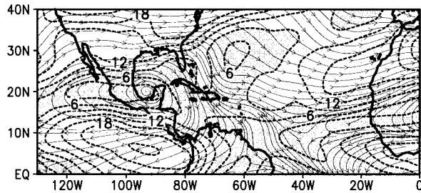
a 200–850 hPa Vertical Shear
