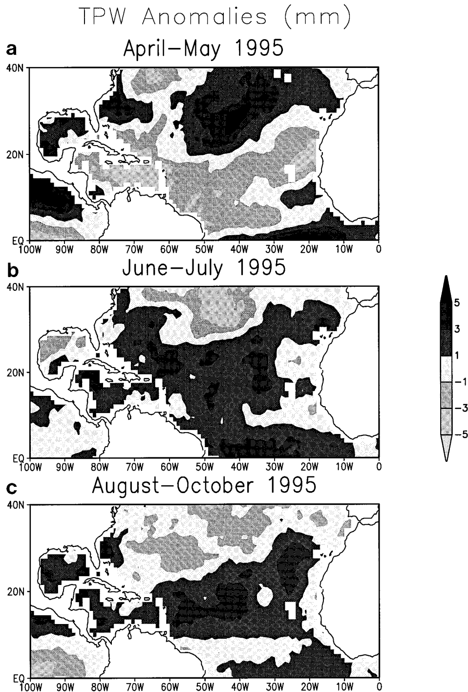
FIG. 9. Total precipitable water (TPW) anomalies (mm) for (a) April–May 1995, (b) June–July 1995, (c) August–October 1995. White areas (near or over land) indicate no analysis possible. Negative anomalies are shaded moderately dark through lightly shaded and positive anomalies are shaded dark. The anomalies are departures from the July 1987–October 1994 base period monthly means.
