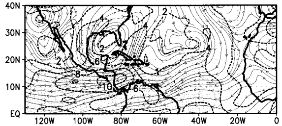
b Vertical Shear Vector
