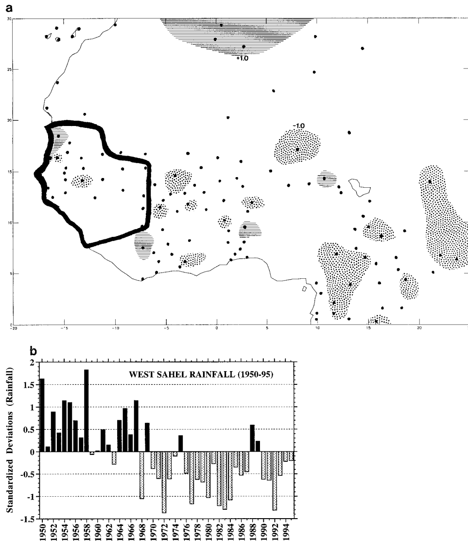
FIG. 12. Standardized anomalies of June–September precipitation from the base period of 1950–90: (a) over North Africa during 1995 and (b) averaged over the western Sahel for each of the 1950–95 seasons. In panel (a) horizontal hatching indicates totals exceeding one standard deviation above normal, and dotted shading indicates totals more than one standard deviation below normal. Station locations are indicated by the dots. The dark curve indicates the Western Sahel region (Landsea et al. 1997). Yearly values in panel (b) are the average of the available station anomalies from a possible 7 stations.
