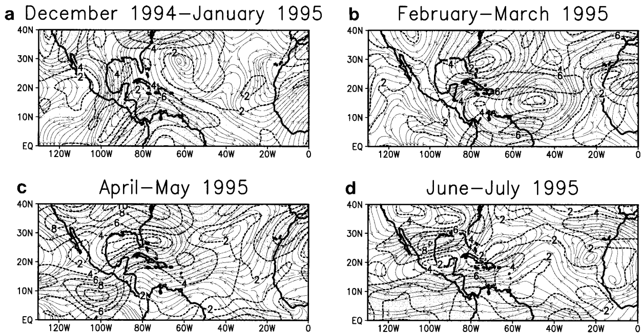
FIG. 6. Same as Fig. 4b except for (a) December 1994–January 1995, (b) February–March 1995, (c) April–May 1995, (d) June–July 1995.
