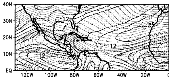
FIG. 2. August–October climatological mean fields: (a) tropospheric vertical wind shear (200 minus 850-mb flow with a contour interval of 3 \text{ m s}^{-1} , with shear values less than 9 \text{ m s}^{-1} shaded); (b) 200-mb streamlines and zonal wind speeds [contour interval of 3 \text{ m s}^{-1} , with positive (negative) values solid (dashed) and any easterly component is shaded]; (c) 850-mb streamlines and zonal wind speeds [contour interval of 2 \text{ m s}^{-1} , with positive (negative) values solid (dashed) and any easterly component greater than 6 \text{ m s}^{-1} is shaded]. Climatology is calculated from the 1979–95 base period monthly means.
