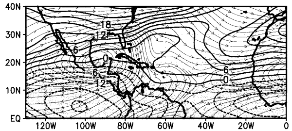
c 850 hPa Streamlines Zonal Wind
