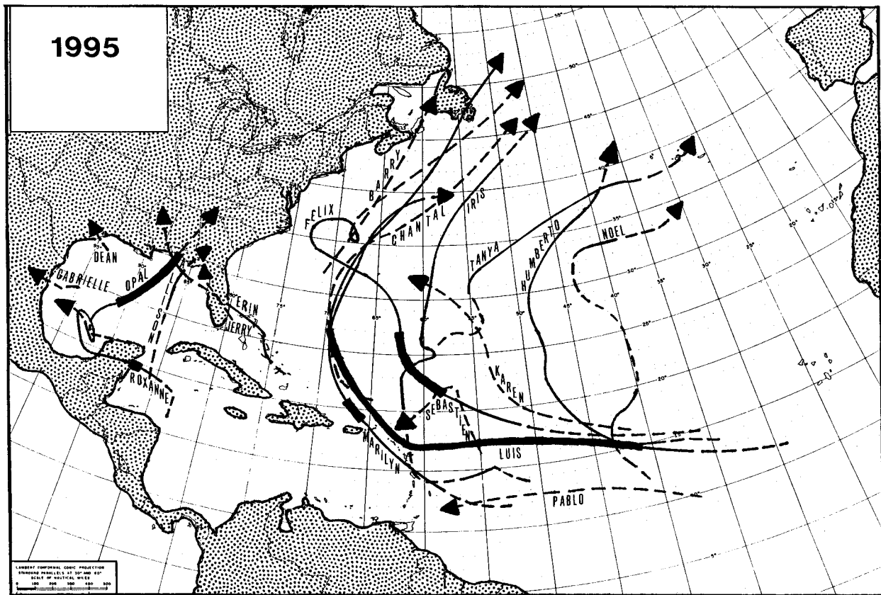
FIG. 1. Tracks of named storms in 1995. Dashed lines indicate the tropical storms (winds 18\text{--}32\text{ m s}^{-1} ), thin solid lines indicate category 1–2 hurricanes (winds 33\text{--}49\text{ m s}^{-1} ), and thick lines show the intense category 3–4–5 hurricanes (winds \geq 50\text{ m s}^{-1} ).
