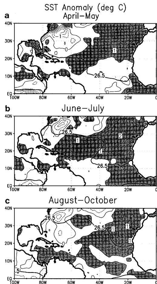
FIG. 8. SST anomalies ( ^{\circ}\text{C} ) for (a) April–May 1995, (b) June–July 1995, and (c) August–October 1995. Contour interval is 0.5^{\circ}\text{C} , with positive (negative) anomalies shown solid (dashed). Values greater than 0.5^{\circ}\text{C} are shaded dark, and values less than -0.5^{\circ}\text{C} are shaded light. The 26.5^{\circ}\text{C} SST contour is also drawn. Anomalies are departures from the 1950–79 base period monthly means.
