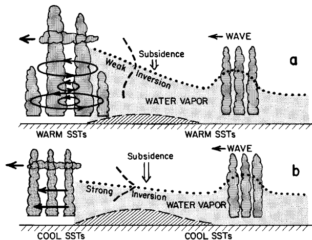
FIG. 17. Idealized schematic of an Atlantic easterly wave disturbance moving westward from Africa into the central and western Atlantic Ocean near 15^{\circ}\text{N} during late summer. In the top diagram (a) only weak surface pressure, warm SSTs, and weak subsidence drying conditions exist. A weak trade wind inversion is present. The top of the moisture level is high enough such that the wave's upward vertical motion is able to overcome the subsidence drying and a tropical cyclone is able to form. In the bottom diagram (b) surface pressure and subsidence are stronger than normal, the SSTs are cooler than normal, the height of the moist level is lower than normal, and the trade wind inversion is stronger. The wave's upward vertical motion cannot overcome these adverse influences. The westward moving easterly wave disturbance of diagram (b) is not able to transform itself into a tropical cyclone and continues to move to the west as a cloud cluster.
