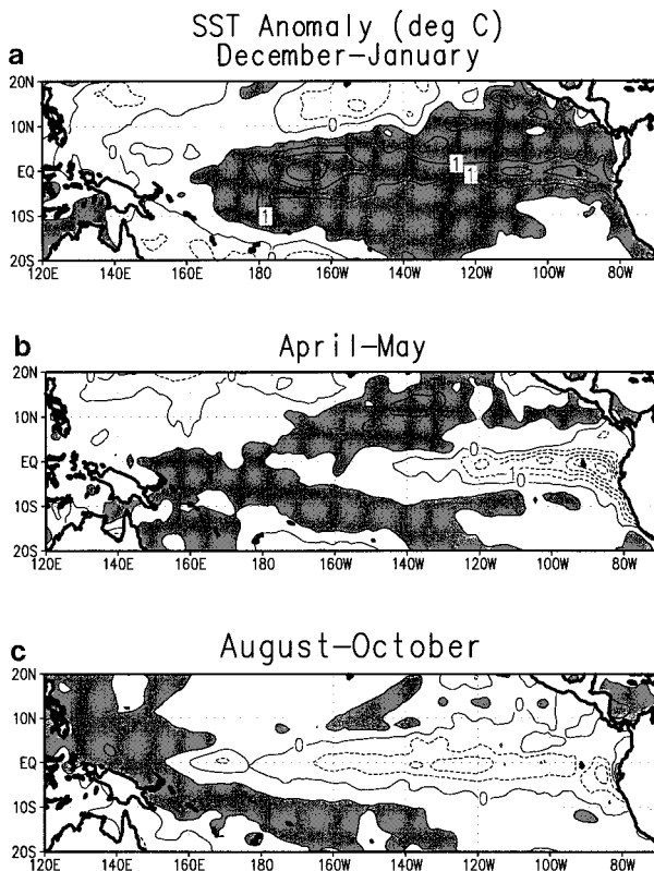
FIG. 11. Tropical Pacific SST anomalies ( ^{\circ}\text{C} ) for (a) December 1994–January 1995, (b) April–May 1995, and (c) August–October 1995. Contour interval is 0.5^{\circ}\text{C} , with positive (negative) anomalies shown solid (dashed). Values greater than 0.5^{\circ}\text{C} are shaded dark, and values less than -0.5^{\circ}\text{C} are shaded light. Anomalies are departures from the 1979–95 base period monthly means.
