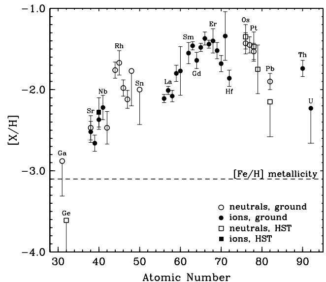
FIG. 3.—Abundances with respect to the Sun [\text{X}/\text{H}] vs. atomic number for elements with Z > 30 . The symbols are defined in the figure, and as in Fig. 1 a dashed line represents the [\text{Fe}/\text{H}] metallicity of CS 22892-052. Detected elements are shown with complete error bars, and upper limits are shown with only the lower half of an arbitrary length error bar. A few element symbols are marked to help with identification of the points. [See the electronic edition of the Journal for a color version of this figure.]
