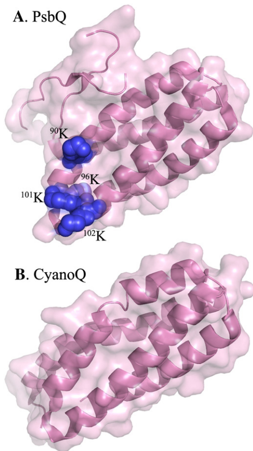
Fig. 4. Crystal Structures of PsbQ and CyanoQ. A., The spinach 1.49 Å PsbQ crystal structure (PDB ID: 1VYK [127]) is shown. The lysyl residues identified by Meades et al. [136] as being involved in electrostatic interaction with PS II are shown in blue. B. The Synechocystis 6803 1.8 Å CyanoQ crystal structure (PDB ID: 3LSO [128]) is shown.
