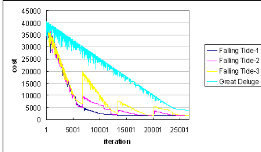
Figure 3. Comparison of a great deluge algorithm and our falling tide algorithm (with N_{run}=3 for the Mar instance)
