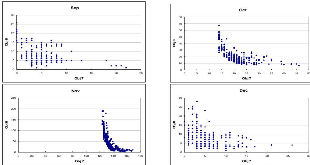
Figure 4. Plots of the non-dominated solutions in terms of objectives 7 and 8
