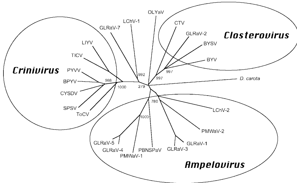
Fig. 4. Phylogenetic tree showing the relationships between the species and genera of the family Closteroviridae based on the sequence of the HSP70 gene. The neighbour-joining tree was produced and bootstrapped using CLUSTAL W. Branch lengths are proportional to sequence distances. GLRaV-7 , LChV-1 , and OLYaV are unassigned species in the family
