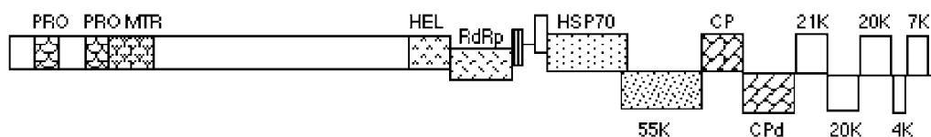
Fig. 2. Genome structure of Grapevine leafroll-associated virus 3 (GLRaV-3) the type species of the genus Ampelovirus , showing the relative position of the ORFs and their expression products. PRO , papain-like protease; MTR , methyltransferase; HEL , helicase; RdRp , RNA polymerase; HSP70 , heat-shock-related protein; CP , coat protein; CPd , divergent coat protein analogue
