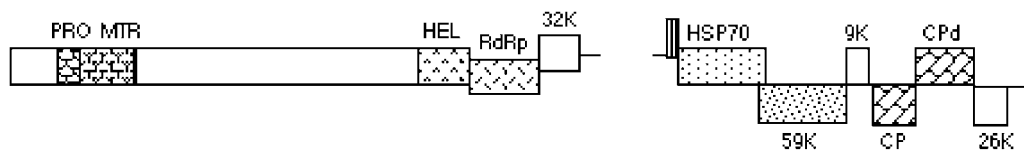
Fig. 3. The bipartite genome structure of Lettuce infectious yellows virus (LIYV), the type species of the genus Crinivirus , showing the relative position of the ORFs and their expression products. PRO , papain-like protease; MTR , methyltransferase; HEL , helicase; RdRp , RNA polymerase; HSP70 , heat-shock-related protein; CP , coat protein; CPd , divergent coat protein analogue
