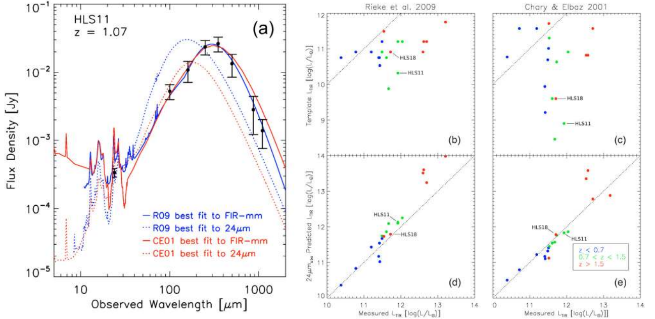
Fig. 2. Left panel a): SED template fits to HLS11, a redshift z \sim 1 LIRG. The data points have been de-magnified by a factor of 1.4 based on our lensing models of the foreground cluster. Although both the R09 and the CE01 templates predict the IR luminosity based on observed 24 \mu\text{m} emission to within a factor of 2, the 24 \mu\text{m} -predicted SEDs do not provide reasonable fits to the FIR-mm data. Right top panels b) and c): the IR luminosity of the best-fit template as it corresponds to the local population is plotted as a function of the actual IR luminosity of each galaxy. The SEDs of our sample are better fit by templates corresponding to systematically lower luminosity local galaxies. Right bottom panels d) and e): the 24 \mu\text{m} -predicted IR luminosity is plotted as a function of the actual IR luminosity of each galaxy. Both template families predict reasonable values for the luminosities of the galaxies in our sample, except in the cases of the ULIRGS/Hyper-LIRGS at z > 1.5 . Note that HLS11 & HLS18 (Fig. 1) fall on the trend line even though their SED shapes show significant deviation in b) and c).
