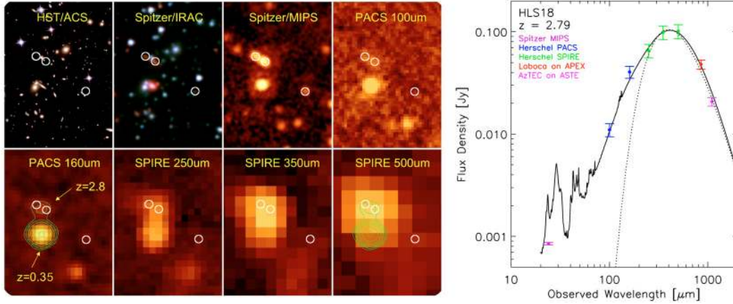
Fig. 1. The most highly magnified galaxy in our sample, HLS18, is the same LIRG first detected by Wilson et al. (2008) with AzTEC at 1.1 mm. Left panel: 1.5' \times 2' thumbnails of the source at a variety of wavelengths highlight the importance of multi-wavelength data to guide the interpretation of the lower resolution maps. IRAC data reveal three lensed images of the galaxy indicated with white circles, although only emission from the two brightest images is detected in the Herschel maps. Right panel: Rieke et al. (2009) SED template fit to the source. The fluxes include the contribution from both of the brightest images of the galaxy, indicated by the two left-most circles in the thumbnails. The data points have not been de-magnified. The 24 \mu\text{m} flux is plotted for reference, although it was not used in the fit. The best-fit modified blackbody is shown with a dotted line and is consistent with previous estimates (Wilson et al. 2008; Gonzalez et al. 2009; Rex et al. 2009).
